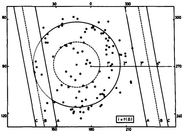
Figure 6.—Distribution of the members of the twin asteroid family Nysa (black dots) and Michela (open circles) in \Omega and i . The center cross is the fundamental plane of the precessional motion of the orbits; the large circles are median values of proper inclination \mu ; the slanting lines are the mean limits of detection on PLS plates in perihelion A , at the mean heliocentric distance B , and in aphelion C .
