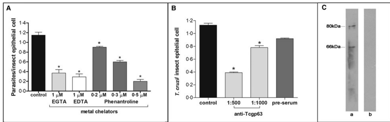
Fig. 2. Effect of divalent metal chelators and anti-Tcgp63-I antibodies on T. cruzi - R. prolixus interaction. Dm28c epimastigotes ( 2 \times 10^7 cells) were treated for 1 h at 27 °C with 1 \mu\text{M} EGTA, EDTA or phenanthroline at 0.2, 0.3 or 0.5 \mu\text{M} (A). Alternatively, the parasites were treated for 60 min at room temperature with anti-Tcgp63-I antibodies at 1:500 and 1:1000 dilution, or pre-immune serum at 1:500 (B). Parasite viability was not affected by the treatments used in this set of experiments. Following interaction for 15 min with the insect gut, the number of adhered parasites/insect gut epithelial cells was estimated by randomly counting at least 100 epithelial cells in quadruplicate in 10 random fields. The results are shown as the mean \pm s.e.m. of two independent experiments. An asterisk denotes significantly different from control (untreated cells) using Student's t test ( *P < 0.001 ). Lastly, western blotting analyses identified two reactive bands against T. cruzi Dm28c epimastigotes (a), while no reactive molecules were recognized by the pre-immune serum (b) (C).
