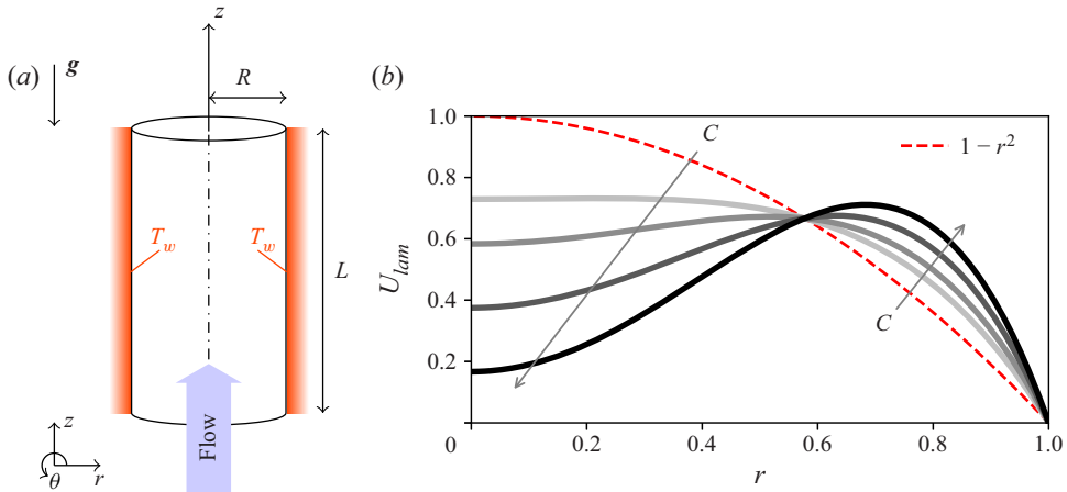
Figure 1. (a) Schematic of the flow configuration. A pipe section of length L and radius R is considered. The pipe is vertically aligned in the gravity field \mathbf{g} and the fluid inside it is driven upwards by an externally applied pressure gradient and by buoyancy. The latter results from the lightening of the fluid close to the heated wall. We assume that the temperature at the wall T_w remains constant in the pipe section. (b) Laminar velocity profiles (2.11a,b) for increasing values of C , as indicated by the arrows. Red dashed line, C = 0 (isothermal profile); light grey to black lines, C = 3, 5, 7.5, 10 .
