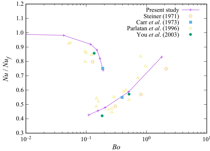
Figure 2. Change in Nu flux, normalised by that for turbulent ‘forced convection’ ( C \rightarrow 0 ), as a function of Bo = 8 \times 10^4 (8NuGr)/(Re^{3.425}Pr^{0.8}) . Data from simulations at Re = 5300 , Pr = 0.7 and various Gr = 16ReC . The upper and lower branches correspond to flow in shear-driven and convection-driven states, respectively.
