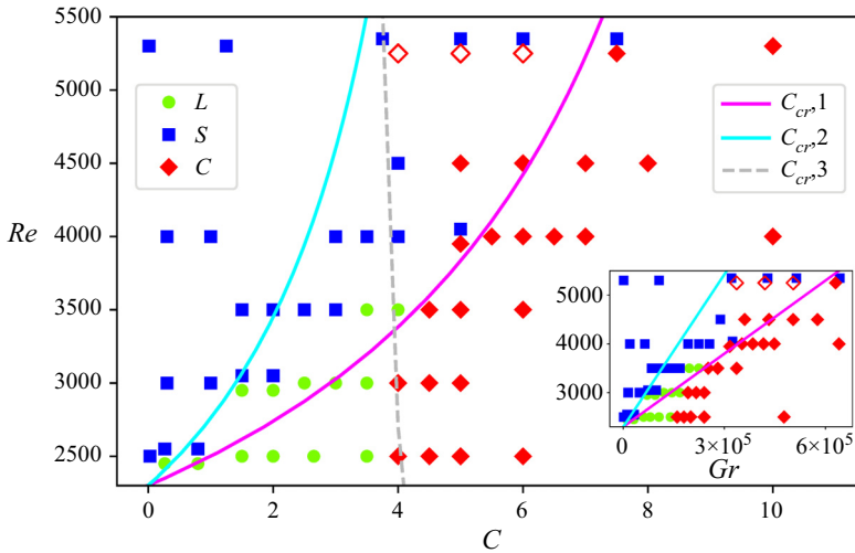
Figure 17. Regions of laminar ( L ) flow, shear-driven ( S ) turbulence and convection-driven ( C ) flow, as in figure 7, together with (3.12) and (3.15) and the linear stability curve (dashed red curve in figure 8). Initial conditions are a shear-driven turbulent state, except for the hollow symbols at Re = 5300 which are started with a convection driven state, and similarly cases towards the bottom-right, where it is clear that the shear-driven state decays immediately.
