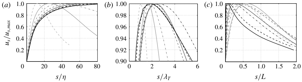
FIGURE 6. Profiles showing the velocity component in the direction of the intermediate principal straining, u_s , along the corresponding s axis (figure 1 a ). The distance to the origin is normalized by the Kolmogorov length scale (a), the Taylor length scale (b) and the integral length scale (c). The legend is the same as that shown in figure 3( d ).
