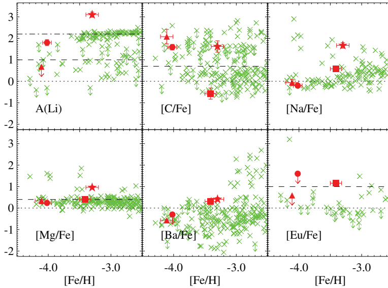
Figure 2. A(Li) vs. [Fe/H] and [X/Fe] vs. [Fe/H] for C, Na, Mg, Ba and Eu. For lithium, the dashed line refers to the average A(Li) among normal red giants with A(Li)~1.0, and the dash-dotted line refers to the observed Li plateau around A(Li)~2.2. For carbon, the dashed line refers to the division of carbon-enhanced and carbon-normal stars with [C/Fe] ~ +0.7. For Mg, the dashed line refers to the canonical value of [\alpha/\text{Fe}] \sim +0.4 for the halo stars. Crosses correspond to literature metal-poor stars. Filled symbols correspond to the peculiar low-metallicity stars discovered and studied with LAMOST and Subaru, with the circle referring to LAMOST J1253+0753, the triangle referring to LAMOST J1313-0552, the square referring to LAMOST J1109+0754 and the star referring to LAMOST J0705+2552. Arrows correspond to upper or lower limits.
