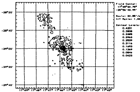
Figure 5-b Cold Fe K-shell transition line (6.4 keV)
