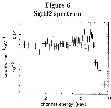
Fig. 6 : The spectrum of Sgr B2 cloud obtained with SIS0 & SIS1.
