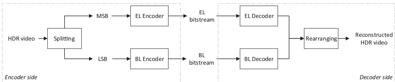
Fig. 5. Dual-layer MSB/LSB splitting architecture.
