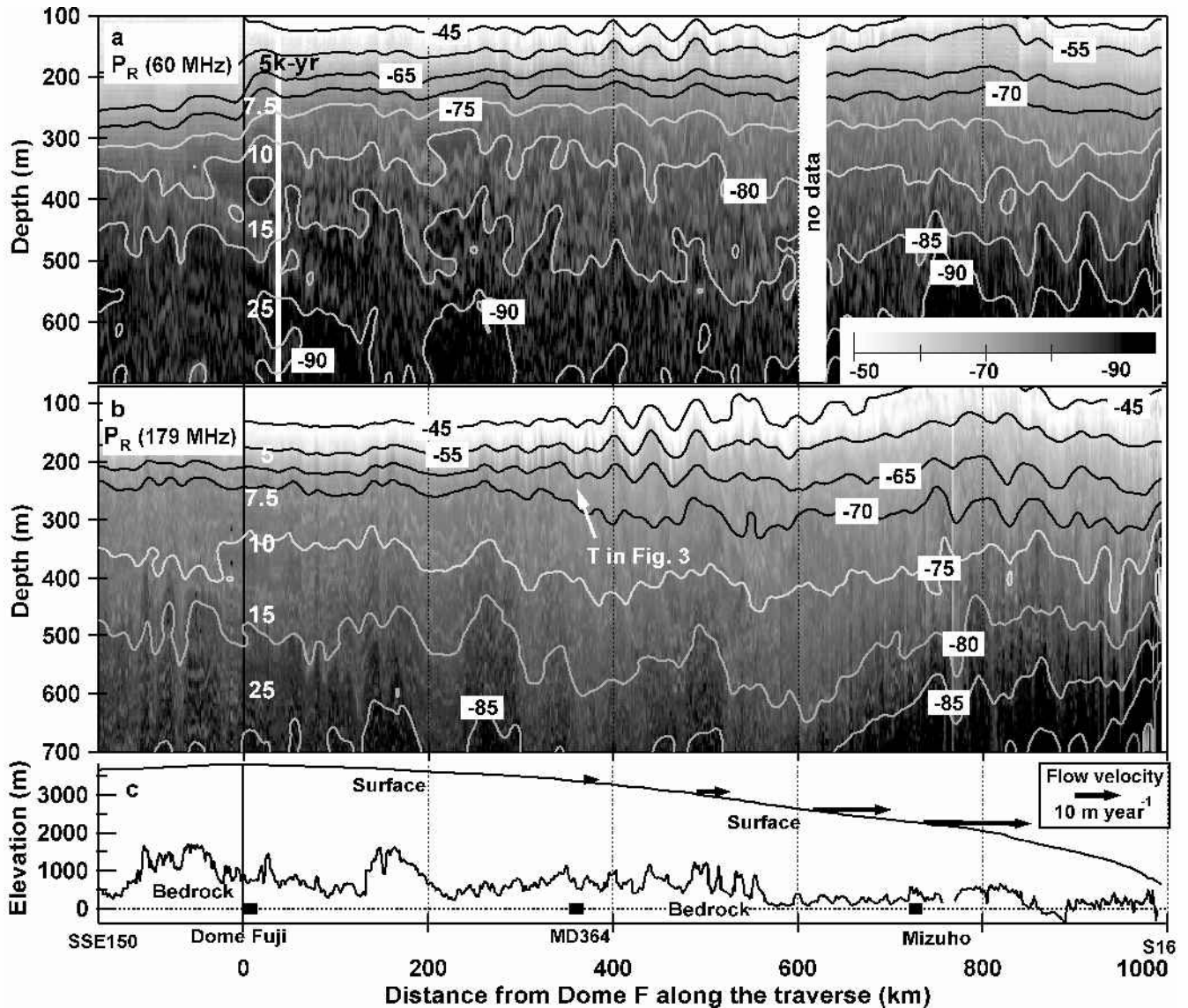
Fig. 2. Distribution of the received power, P_R (dBm) from within the top 100–700 m of the ice sheet along the 1150 km traverse. The upper two density plots are from the 60 MHz radar with a pulse width of 250 ns (upper) and from the 179 MHz radar with a pulse width of 150 ns (lower). A gray scale for the received power is shown at the upper right. The mean trends of uniform P_R are shown by contour lines. The 15 km running averages of uniform P_R are shown as contour lines. The contour interval is halved below the -65 contour. The 60 MHz data between SSE150 and Dome F and above 300 m were affected by internal noise of the radar system, i.e. the lowering of the contour lines in this region is an artifact. Instead, the P_R values should be several dB lower. Internal echoes from strata are often shown as the first derivative of the received power vs depth, but this is not done here because such a filtering process would have caused a loss of information on scattering strength. The age of ice is given at the coring site of Dome F (Watanabe and others, 1999). The bedrock elevation plot at the bottom indicates some correlation between peaks of the bedrock and near-surface contour peaks in P_R . Also shown is the surface elevation, ice-flow velocity and three locations that are imaged in finer detail in Figure 3. The surface elevations are from the European Remote-sensing Satellite-1 (ERS-1) satellite-borne radar altimeter, and the bedrock elevation was measured by the radar sounding.
