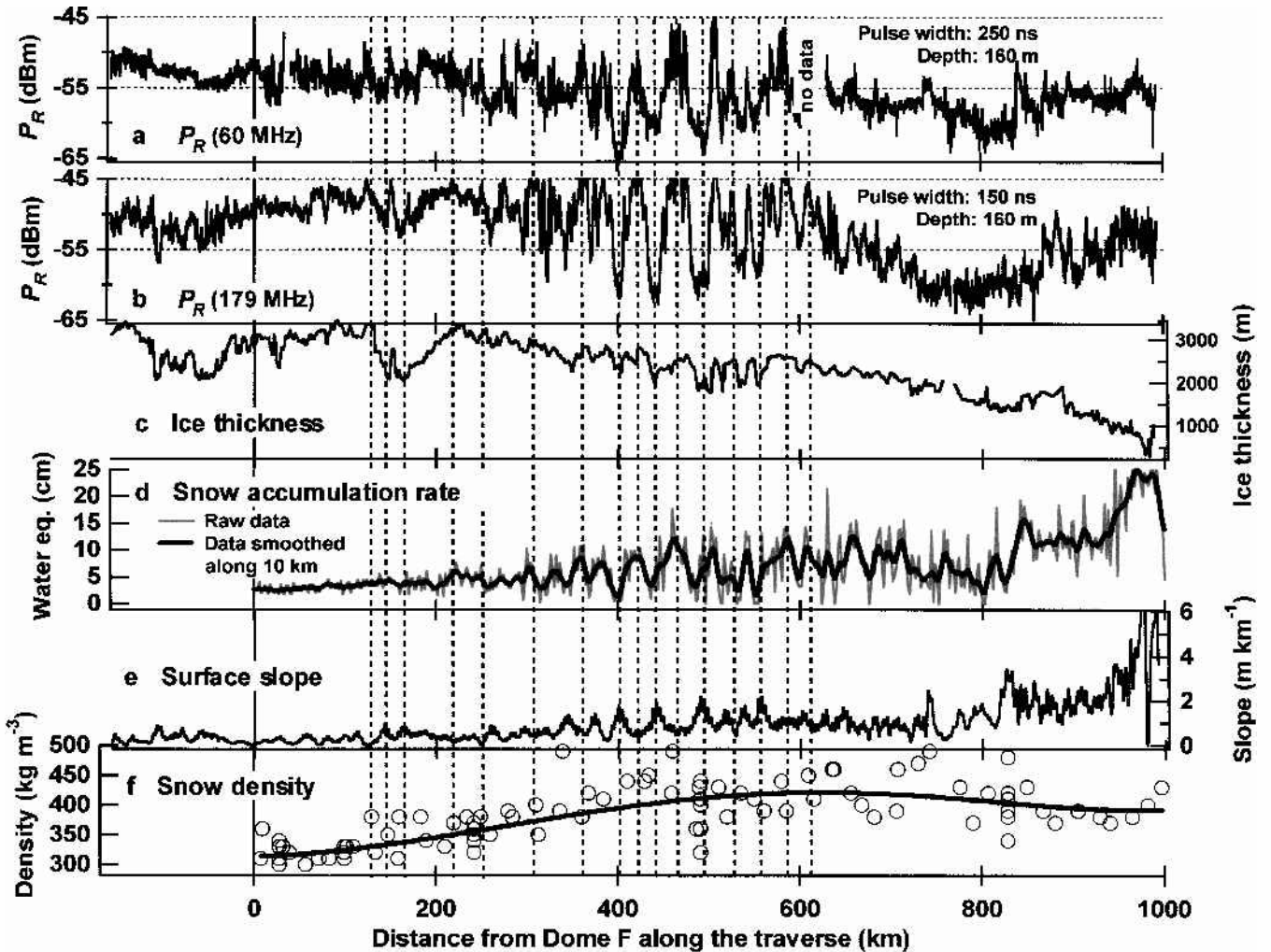
Fig. 5. Radar scattering at 160 m and environmental conditions along the 1150 km traverse. Received power P_R of the 60 MHz radar and the 179 MHz radar scattered from 160 m depth is shown in (a) and (b), respectively. The ice-sheet conditions are as follows: (c) ice thickness; (d) snow accumulation rate (Satow and others, 1999); (e) surface slope along the traverse calculated from the elevation data; (f) density of the snow in the top 20 cm of the ice sheet as measured by a snow sampler and a balance (Azuma and others, 1997; Fujita and others, 1998; Motoyama and others, 1999). The vertical dashed lines indicate the correlations between the profiles. P_R (60 MHz) at sites between SSE150 and Dome F contains a systematic error due to the internal noise of the radar system. It should be a few dB lower.
