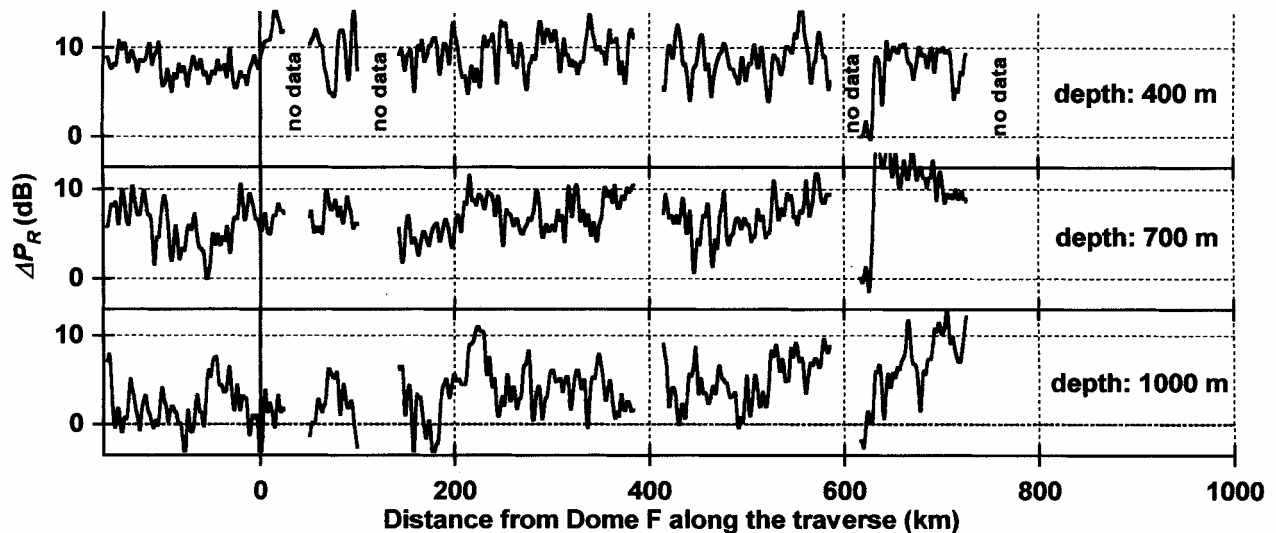
Fig. 4. Variation of \Delta P_R = P_R(179 \text{ MHz}) - P_R(60 \text{ MHz}) along the traverse for depths of 400, 700 and 1000 m. The 179 MHz radar used a pulse width of 350 ns. The dominant reflection mechanism is changes in dielectric permittivity when \Delta P_R is close to 10 dB (Fujita and others, 1999), whereas the dominant reflection mechanism is changes in electrical conductivity when \Delta P_R is close to 0 dB.
