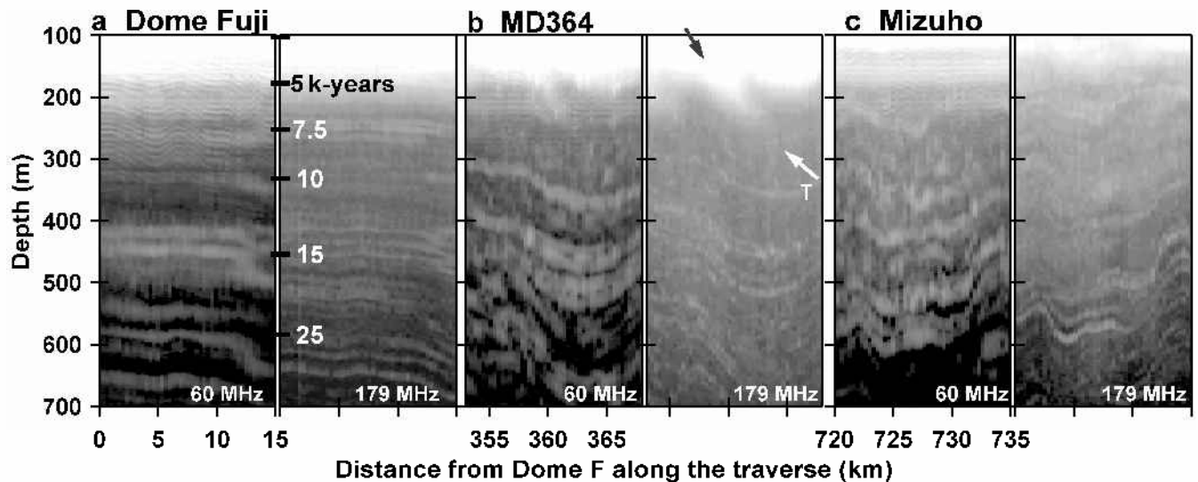
Fig. 3. Finer-scale features of the received power P_R along the three 15 km long cross-sections marked in Figure 2. Gray scales for the power are the same as in Figure 2. These density plots indicate continuity and stability of stratified structure of the scatterers near the dome summit compared with the downstream regions. The very thin striped interference pattern in the top 300 m of the 60 MHz data is due to internal noise of the radar system. The age of ice is given at the coring site of Dome F (Watanabe and others, 1999). The arrows labeled “T” indicate an example of the suggested trajectories.
