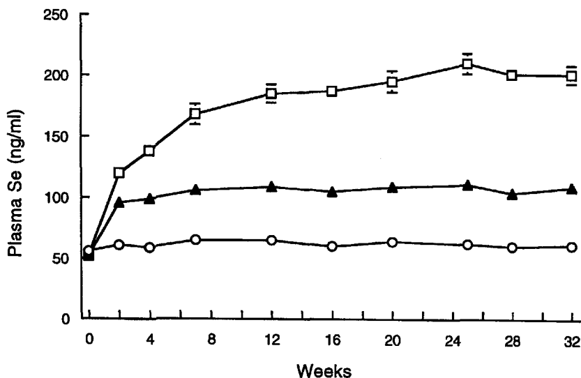
Fig. 2. Selenium concentrations in plasma of New Zealand women supplemented with selenium either as selenate (▲, n 10), or Se-enriched yeast (□, n 12), or a placebo (○, n 9) for 32 weeks. For details of dietary treatment see p. 552. Values are means and their standard errors represented by vertical bars.
