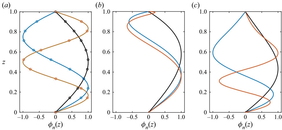
Figure 3. Mode shapes in a uniform stratification with an exponential background velocity profile (3.1) for (a) Ri = \infty (continuous lines, no shear), Ri = 10^5 (hollow circles, weak shear), (b) Ri = 1 (finite shear, cograde modes) and (c) Ri = 1 (finite shear, retrograde modes). In each panel, mode numbers n = 1 (black), 2 (blue) and 3 (red) are shown.
