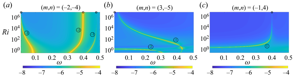
Figure 8. Contour plot of \log_{10}[\bar{h}_{mn}^{max}] similar to figure 5 but for representative (a) retrograde modal interaction (m, n) = (-2, -4) , (b) mixed modal interaction (m, n) = (3, -5) , and (c) mixed modal interaction (m, n) = (-1, 4) , plotted on the plane of primary wave frequency \omega on the x-axis and Richardson number Ri on the y-axis. Hollow circles at Ri = 10^7 indicate the locations of divergence calculated from weak shear asymptotic theory. The mode number of the superharmonic internal wave at the divergence locations is indicated by the encircled numbers next to the corresponding divergence curves. The negative sign before mode number indicates that it is a retrograde mode.
