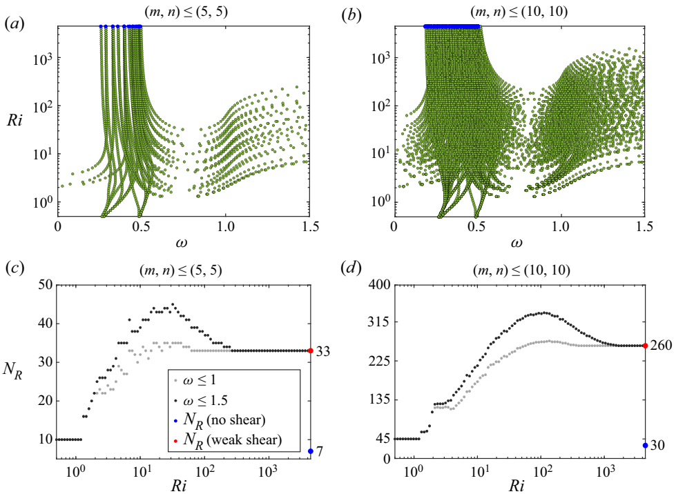
Figure 7. Resonance locations for all the cograde modal interactions amongst (a) (m, n) \leq (5, 5) and (b) (m, n) \leq (10, 10) , in the plane of primary wave frequency \omega and Richardson number Ri . Number of resonance locations ( N_R ) shown at different Richardson numbers ( Ri ) for all the cograde modal interactions (c) (m, n) \leq (5, 5) and (d) (m, n) \leq (10, 10) . In (a,b), blue dots indicate the resonance locations in the weak shear limit ( Ri \rightarrow \infty ). In (c,d), the red and blue dots indicate N_R in the weak shear and no shear limits, respectively.
