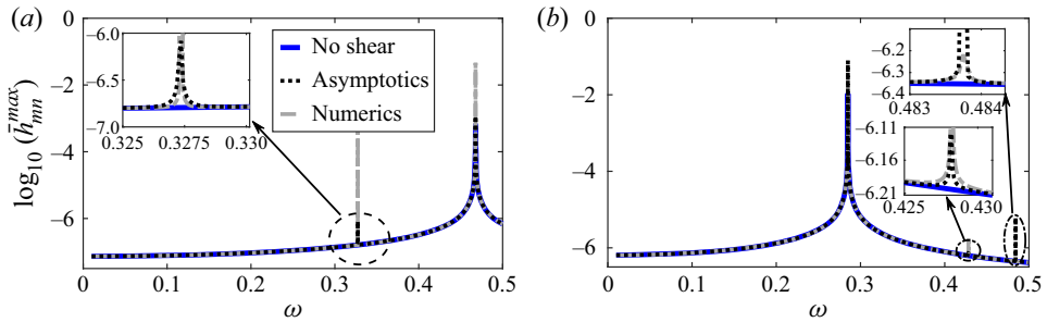
Figure 4. Superharmonic wave amplitude \log_{10}[\bar{h}_{mn}^{max}] (2.12) plotted as a function of primary wave frequency \omega at Ri = \infty (no shear, shown in blue) and Ri = 10^7 (asymptotics, numerics), for representative modal interactions specified by (m, n) = (a) (2, 3), (b) (2, 5) . The insets show a zoomed-in view of the additional divergences that occur in the presence of weak shear.
