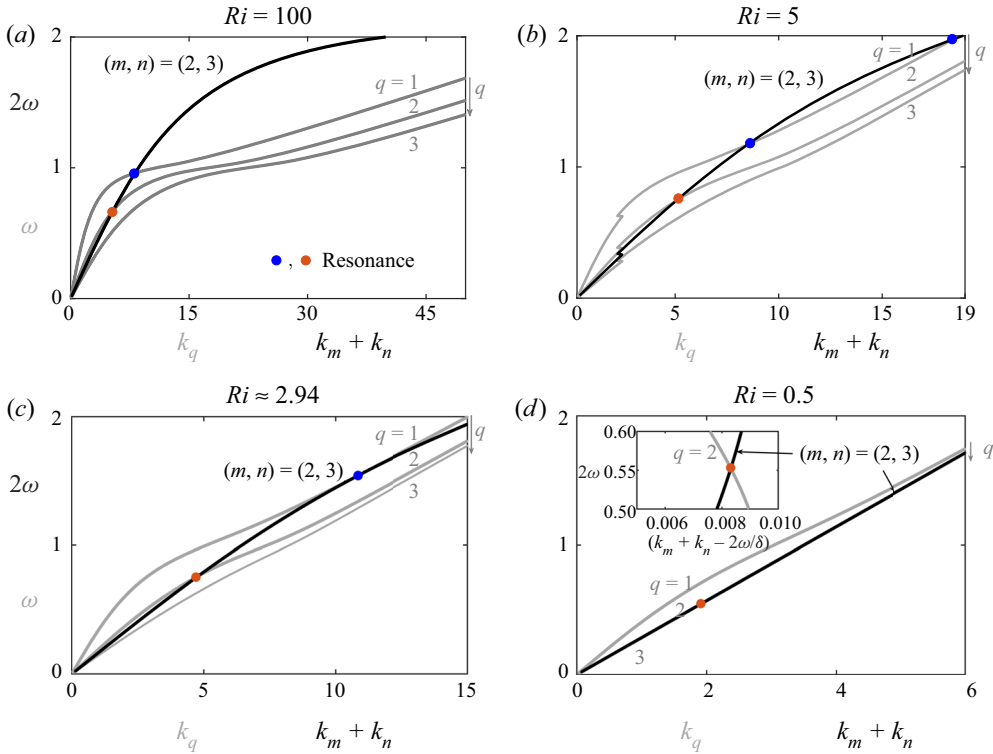
Figure 6. Dispersion curves for mode numbers q = 1 to 3 (grey lines) for (a) Ri = 100 , (b) Ri = 5 , (c) Ri \approx 2.94 and (d) Ri = 0.50 . The black solid lines represent 2\omega vs (k_m + k_n) with (m, n) = (2, 3) . Points of intersection with the mode-1 and mode-2 superharmonic dispersion curves are indicated by the blue and red dots, respectively. In (d), the inset shows a zoomed-in view (with a modified quantity on the x-axis for better clarity) around the intersection point denoted by the red dot.
