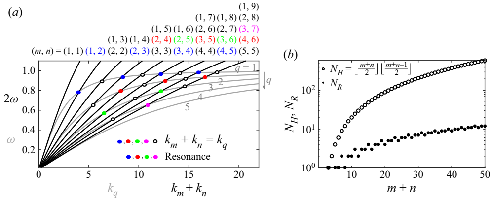
Figure 1. (a) Dispersion curves ( \omega vs k_q , grey lines) for mode numbers q = 1, 2, 3, 4, 5 in a uniform stratification with no shear. The black lines show 2\omega vs k_m + k_n for m + n = 2 to 10 , with modes m and n being at frequency \omega . Horizontal resonance condition k_m + k_n = k_q is satisfied at the points of intersection (filled and unfilled circles). Filled circles represent actual resonances. (b) Number ( N_H , unfilled circles) of modal interactions (between modes m and n at frequency \omega , 0 < \omega < 0.5 ) for which the horizontal resonance condition k_m + k_n = k_q (mode q being at 2\omega ) is satisfied, plotted as a function of m + n . Number N_R (filled circles) from the N_H modal interactions that are also resonances. The symbol \lfloor \rfloor refers to the floor operator.
