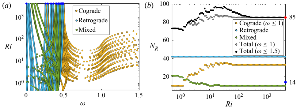
Figure 9. (a) Resonance locations for all the modal interactions amongst (|m|, |n|) \leq (5, 5) i.e. for cograde, retrograde and mixed interactions, in the primary wave frequency \omega and Richardson number Ri plane. The blue dots indicate resonance locations in the weak shear limit. (b) Number of resonance locations ( N_R ) plotted as a function of Richardson number ( Ri ) for all the modal interactions amongst (|m|, |n|) \leq (5, 5) . The red and blue dots indicate the total number of resonance locations in the weak shear and no shear limits, respectively.
