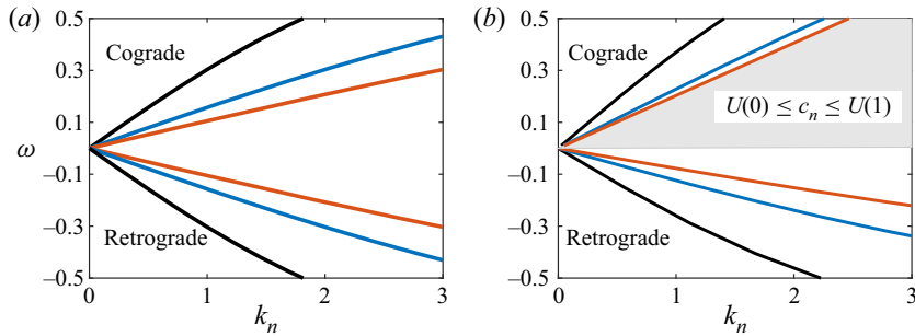
Figure 2. Dispersion curves for different mode numbers in a uniform stratification for (a) Ri = \infty and (b) Ri = 1 . In each panel, the black, blue and red colours correspond to mode numbers n = 1, 2 and 3 , respectively.
