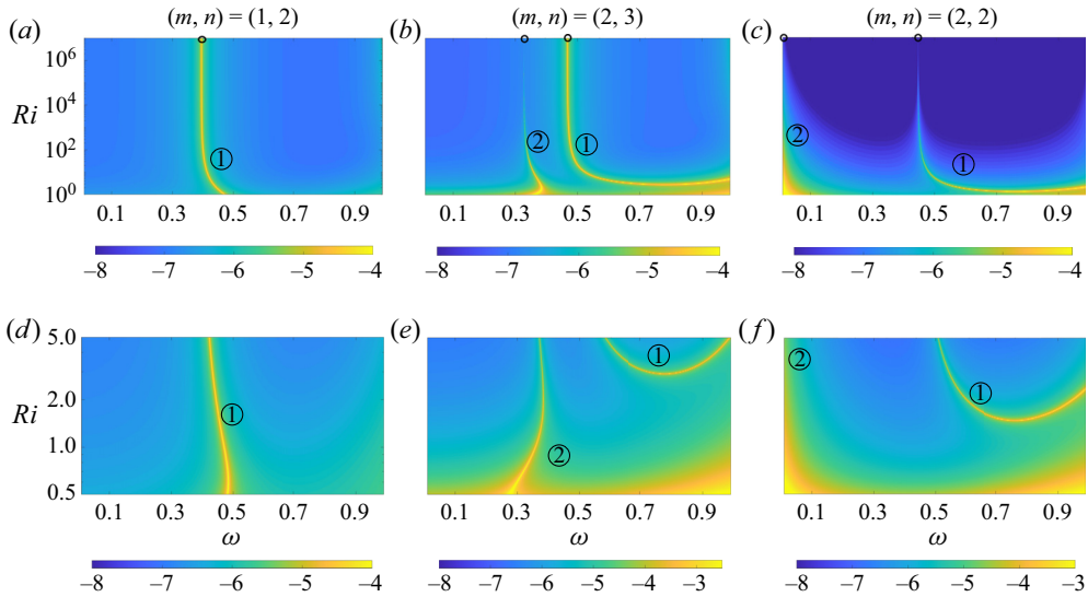
Figure 5. Contour plot of \log_{10}[\bar{h}_{mn}^{max}] for (m, n) = (a) (1, 2), (b) (2, 3), (c) (2, 2) , plotted on the plane of primary wave frequency \omega on the x -axis and Richardson number Ri on the y -axis. Hollow circles at Ri = 10^7 indicate the locations of divergence calculated from weak shear asymptotic theory. The mode number of the superharmonic internal wave at the divergence locations is indicated by the encircled numbers next to the corresponding divergence curves. Panels (d–f) are zoomed-in views of (a–c), respectively, in the regions of small Ri .
