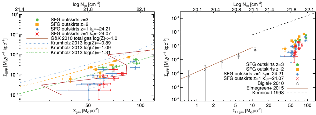
Figure 2. Left: Comparison of the SFR efficiency of DLA gas in the outskirts of SFGs at z \sim 1-3 with the z \sim 3 simulation by Gnedin & Kravtsov (2010) and the analytic KMT+ model by Krumholz (2013). The KMT+ model predictions are for the metallicities of DLAs at the redshifts of the binned SFGs, with the colors matching those of the corresponding measurements at each redshift: green for z=3 , orange for z=2 , and blue for z=1 . The model provides a measure of the expected evolution in the SFR as a function of redshift due to the metallicity evolution of DLAs, which would evolve from the green line at z = 3 to the blue line at z = 1 . The data are broadly in agreement with the simulations and models, although the data do not reproduce the predicted metallicity evolution. Right: Comparison of the SFR efficiency of DLA gas in the outskirts of SFGs at z \sim 1-3 with local measurements. This shows that the upper limits from direct DLA observations are consistent with both our measurements and the local HI gas.
