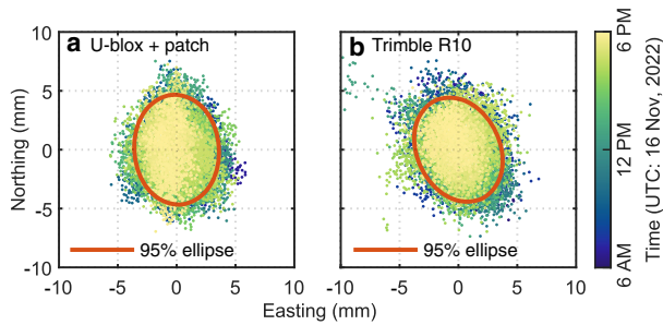
Figure 4. Horizontal positions and 2D 95% confidence ellipses for the u-blox and Trimble position time series. Confidence ellipses are computed from n = 43,200 positions obtained over 12 hours on 16 November, 2022. ‘North’ corresponds to grid north and the coordinate system is the same as in Fig. 3.
