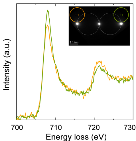
Figure 2. EEL spectra showing a dichroic signal at the Fe L_{3/2} absorption edges. The inset the diffraction pattern under three beam conditions. The areas, from which the EEL spectra are collected, are marked with circles.
