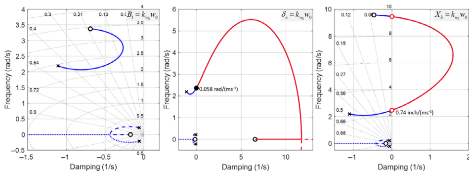
Figure 14. FXV-15 at 95kts in C-mode, nacelle angle 60deg, flap 40deg, descent angle 3.5deg; eigenvalue loci for varying gain k_{w_0} with feedback to cyclic B_1 , elevator \delta_e and pilot's stick X_b .
