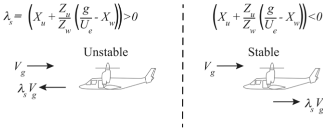
Figure 7. Surge mode stability either side of the minimum power speed.
