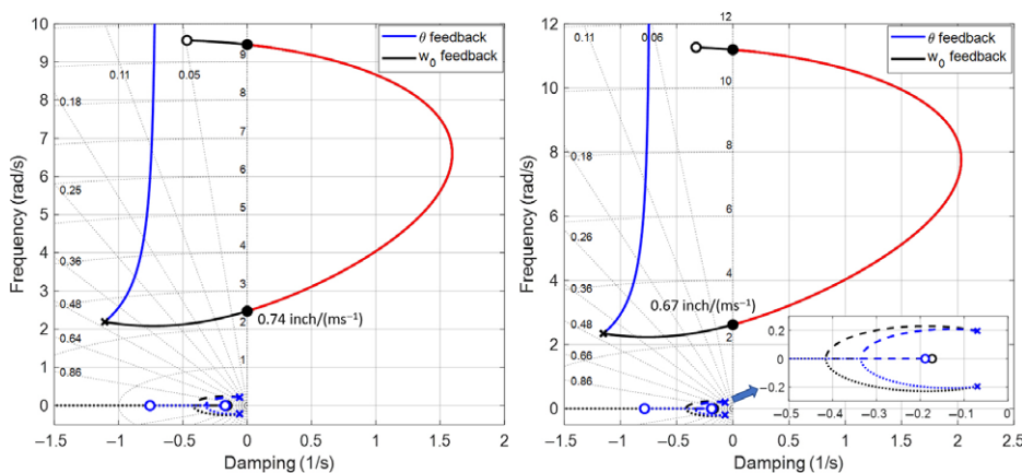
Figure 15. Eigenvalue loci showing comparison between pitch attitude and vertical velocity feedback; FXV-15 in C-mode with 60deg nacelle, 3.5deg descent at 95kts and 105kts.
