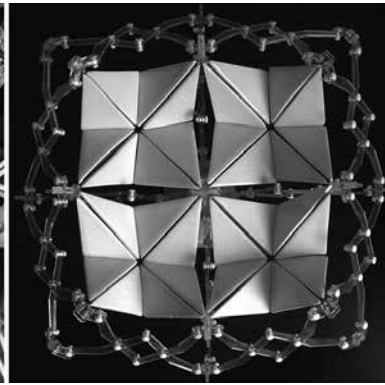
5 a, b Kinetic solar facade by J. Fosbrook, A. John, O. O'Neil, 2012.
