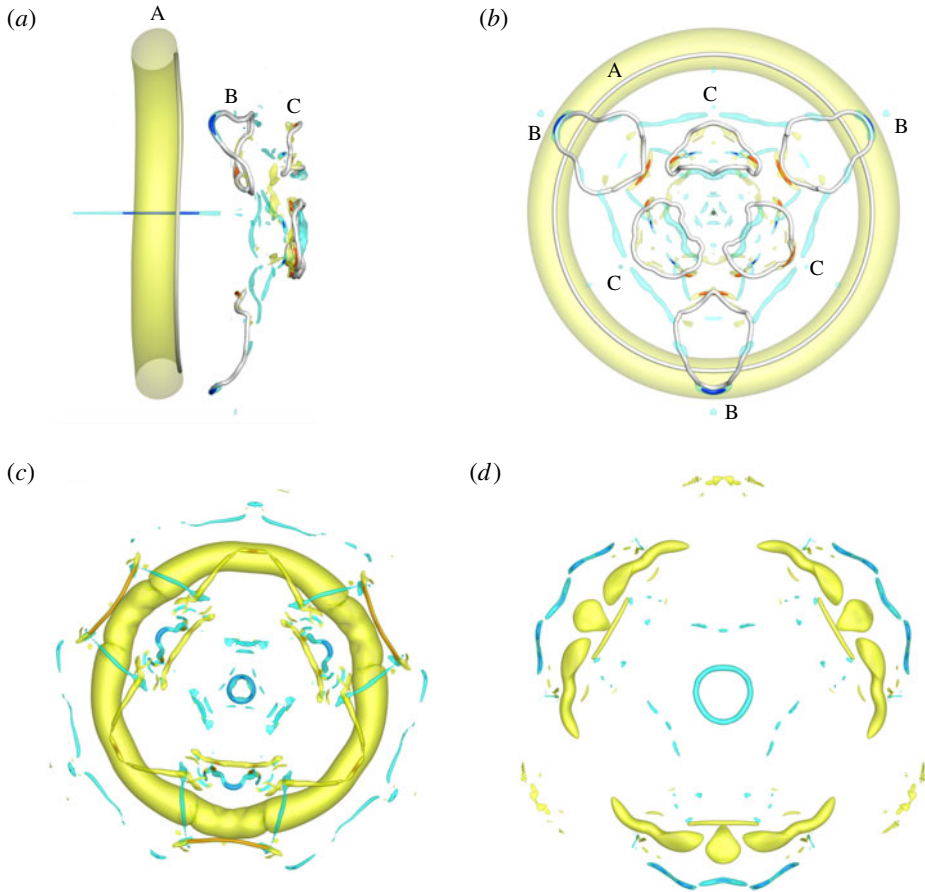
FIGURE 12. (Colour online) Iso-surfaces of \omega_s at Re = 27\,000 in the randomly perturbed ring. (a) Side view at t=6 , and (b), (c) and (d) top views at t=6 , 10 and 12 respectively. Blue, cyan, yellow and red colours represent \omega_s = -10, -5, 5 and 10 in (a), (b) and (c), and \omega_s = -16, -8, 8 and 16 in (d). Circular lines denote vortex lines.
