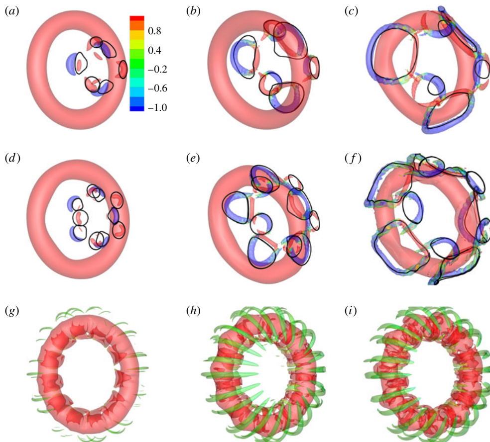
FIGURE 6. (Colour online) Iso-surfaces of \lambda_2 = -0.5 , coloured by \omega_s , at t = 4, 6 and 8 from left to right. The ringlets are delineated by vortex lines (circular lines in a-f ). The initial perturbation is optimal at m = 3, 5 and 11 in the top, middle and bottom rows.
