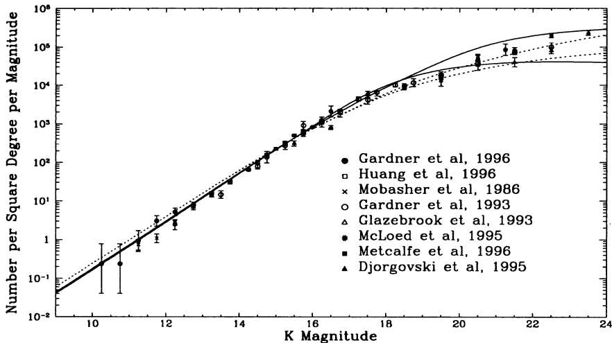
Figure 2. The K-band number counts with models based upon our luminosity functions. The solid lines include the effects of passive evolution, the dotted lines are pure K-correction models. The higher line in each case is for q_0 = 0.02 , while the lower lines are for q_0 = 0.5 . References for the data are given in Gardner et al. (1996).
