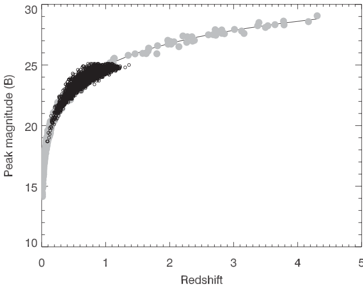
Figure 1. Projected Hubble diagram for Type Ia supernovae including simulated data from E-ELT and EUCLID. The grey circles with z < 1 represent the sample that already exists, or will exist within the next few years. These are almost entirely optical observations. The potential sample of SNe with NIR measurements from EUCLID are shown as black dots (simulated data provided by K. Maguire). The circles with z > 1 represent the sample that could be obtained with a combination of JWST imaging and E-ELT spectroscopic follow-up.
