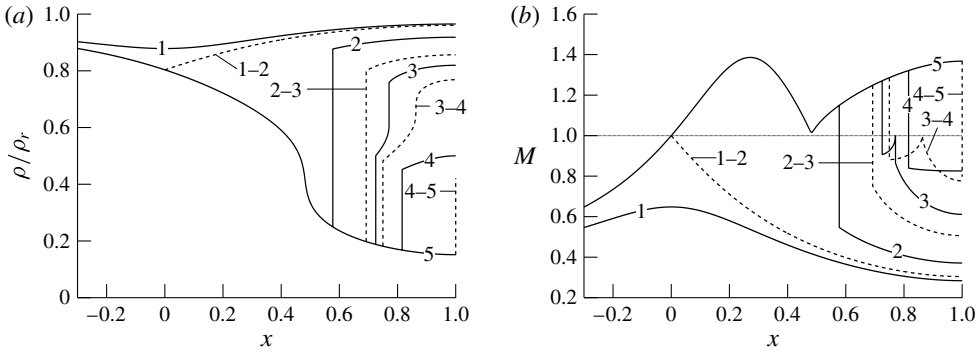
FIGURE 14. Exemplary limiting (---) and intermediate (—) flows of type \mathcal{R}_0^{NC} , computed from the van der Waals polytropic model with c_v/R = 50 . (a) Density solutions, scaled to reservoir density \rho_r ; (b) Mach number solutions. Reservoir conditions: P_r = 1.2315P_c , v_r = 0.7287v_c .
