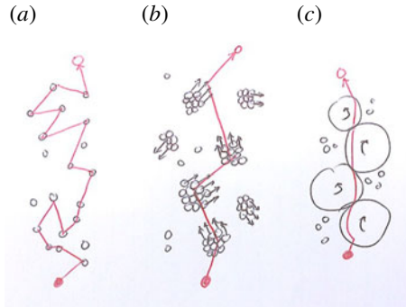
FIGURE 1. Sketch of three modes of mass transport: (a) diffusion, (b) convection via clusters and (c) ‘rotoction’, i.e. rotations of clusters mediating convection in dense shear flow as found by Macaulay & Rognon (2019).
