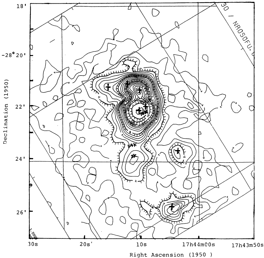
Fig. 1. 43 GHz continuum map of the Sgr B2 region with a 38" resolution. The components MD1 through MD7 are shown by + marks from right to left in the map.
