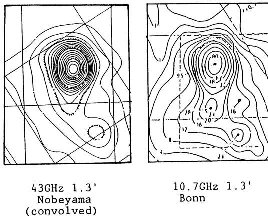
Fig. 2. Continuum maps of the Sgr B2 core region at 43 GHz (left; convolved to a 1.3' resolution) and at 10.7 GHz (right; reproduced from Downes et al. 1978).
