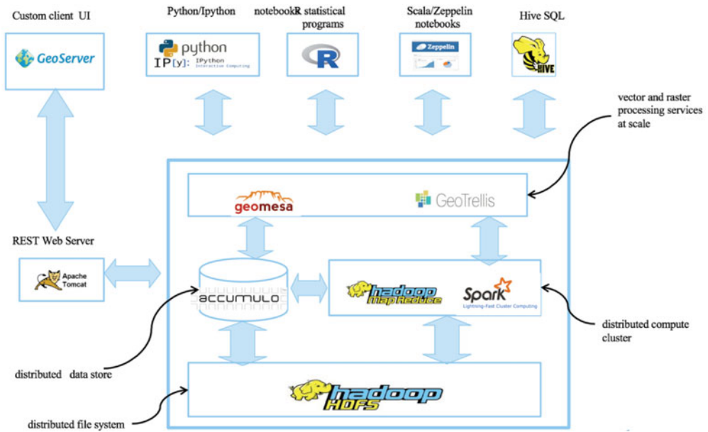
Figure 2. Architecture for the Water Management stack. Accumulo as the DB, HDFS forming the backup, mapreduce and Spark powering the computation, and GeoMesa/GeoTrellis providing the indexing; various webservices and Python/R providing the interfaces.
