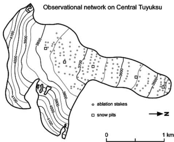
Fig. 2. Topography and observational network of central Tuyuksu (from Haeberli and others, 2001).
