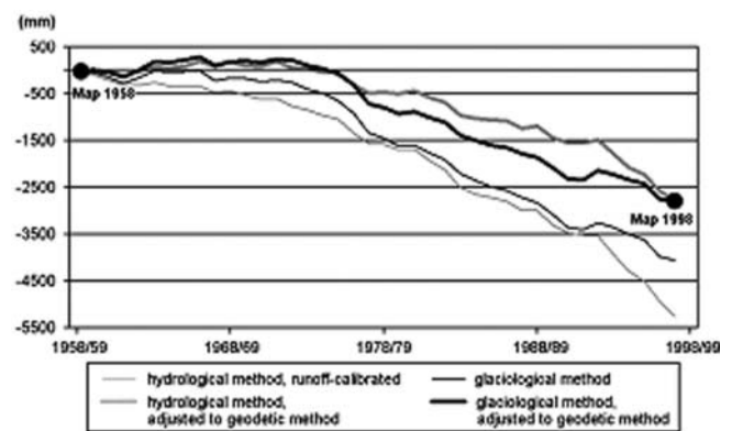
Fig. 5. Specific mass-balance curves for the catchment of the gauging station 'Tourist Camp Tuyuksu', derived by the hydrological and glaciological method, before and after the adjustment to the geodetic method.
