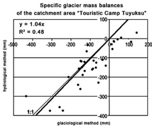
Fig. 4. Scattergram of specific glacier mass balances derived by the hydrological method and by direct measurements of the years 1958/59 to 1989/90 for the catchment of 'Tourist Camp Tuyuksu'.
