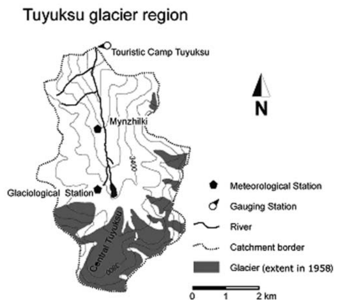
Fig. 1. Schematic sketch of the investigation area.
