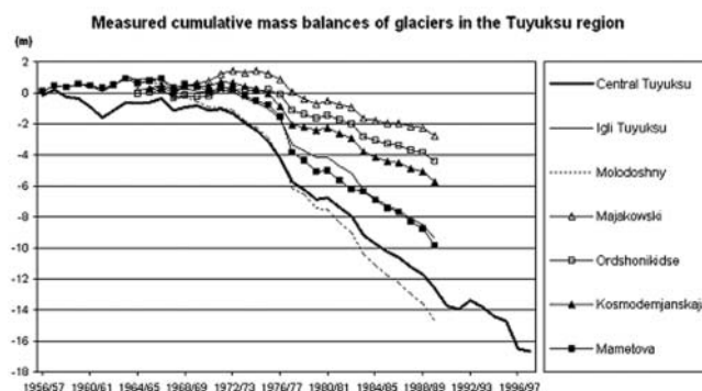
Fig. 3. Cumulative specific mass balances for glaciers in the Tuyuksu region.
