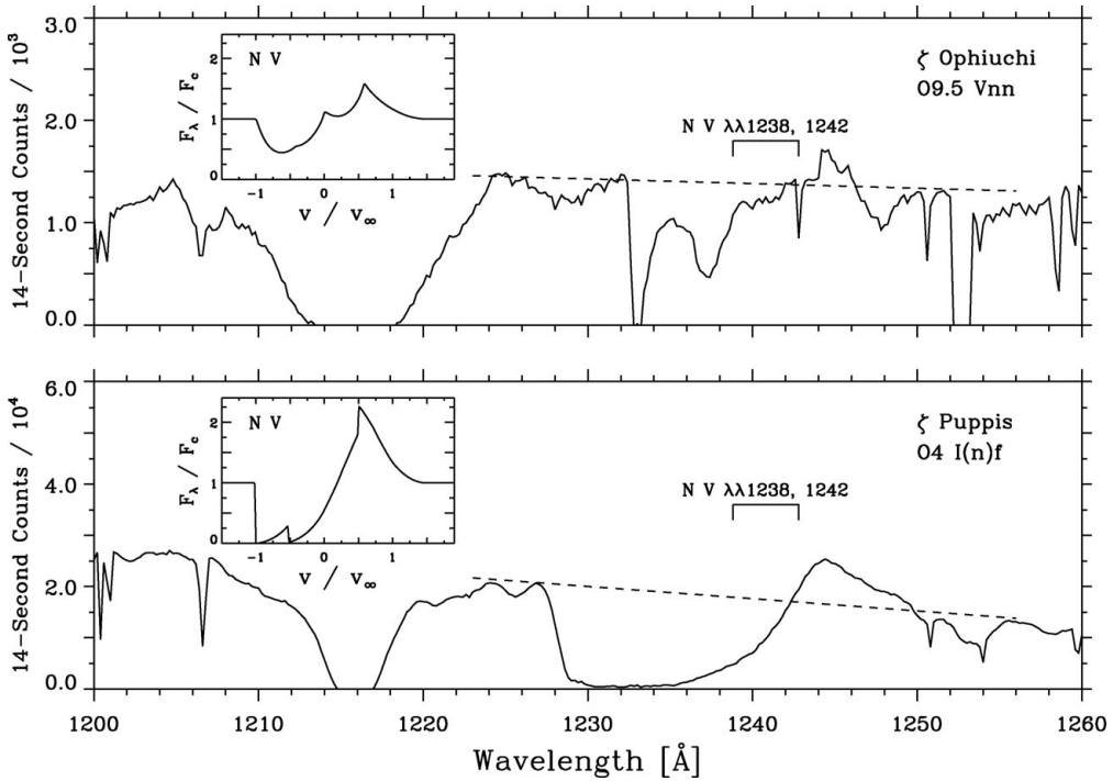
Figure 1. Copernicus spectra of the N V \lambda\lambda 1238, 1242 resonance doublet of \zeta Oph (top) and \zeta Pup (bottom). Inset panels show model predictions from the standard model. Inspired by Fig. 1 of Morton (1976).
