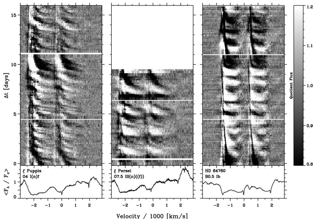
Figure 2. Spectroscopic time series observations of the Si IV \lambda\lambda 1394, 1403 resonance doublet of \zeta Pup (left). \xi Per (middle), and HD 64760 (right). The time series of \zeta Pup and HD 64760 were obtained during the IUE “MEGA Campaign”, while the observations of \xi Per were obtained with IUE in 1994 October. In all cases the dynamic spectra have been normalized by the mean spectrum from the time series.
