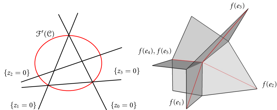
Figure 11: On the left is the conic \mathcal{F}'(\mathcal{C}) from Example 2.12 with its position with respect to the 4 lines in \overline{\mathbb{P}} \setminus \mathcal{P} . On the right the tropicalisation drawn in the compactification \overline{\mathbb{P}} \subset \mathbb{TP}^3 of the standard tropical plane.
