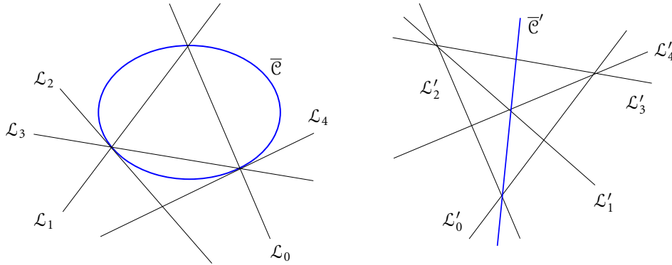
Figure 12: Two compactifications of the plane \mathcal{P} from Example 2.3 along with the compactification of a curve \mathcal{C} \subset \mathcal{P} from Example 3.4.
