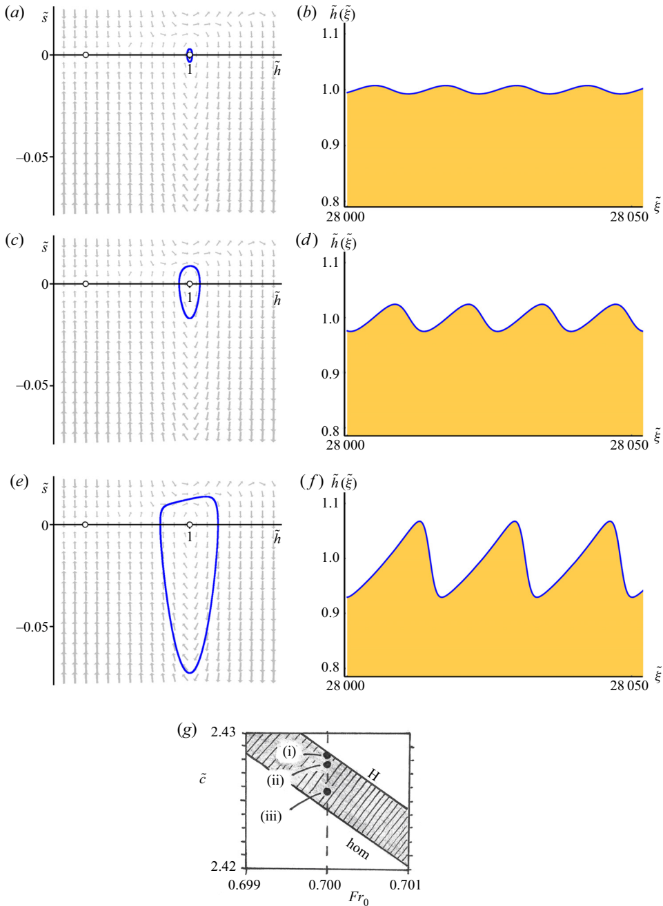
Figure 5. Phase space portraits and corresponding wave profiles for three successive values of \tilde{c} at fixed Fr_0 = 0.7 , as shown in the accompanying section of the (Fr_0, \tilde{c}) parameter plane: (a,b,g(i)) at \tilde{c} = \tilde{c}_H - 10^{-4} = 2.42847 , the limit cycle has just been born from (1, 0) and is still quite symmetric. The waves are nearly sinusoidal and of small amplitude. (c,d,g(ii)) At \tilde{c} = \tilde{c}_H - 10^{-3} = 2.42757 , the limit cycle has become bigger and starts to develop an asymmetry. The roll waves are therefore of larger amplitude and wavelength, and their shape deviates from the harmonic. (e,f,g(iii)) At \tilde{c} = \tilde{c}_H - 4 \times 10^{-3} = 2.42457 , the limit cycle has grown further and now exhibits a marked asymmetry. A practically straight segment appears on its topmost part, which is responsible for the nearly exponential shape of the rising flanks of the roll waves. The latter are now seen to have an even larger amplitude and wavelength. The background grey arrows denote the direction field of the dynamical system. The system parameters are as in table 1 and the inclination angle is \zeta = 36^\circ .
