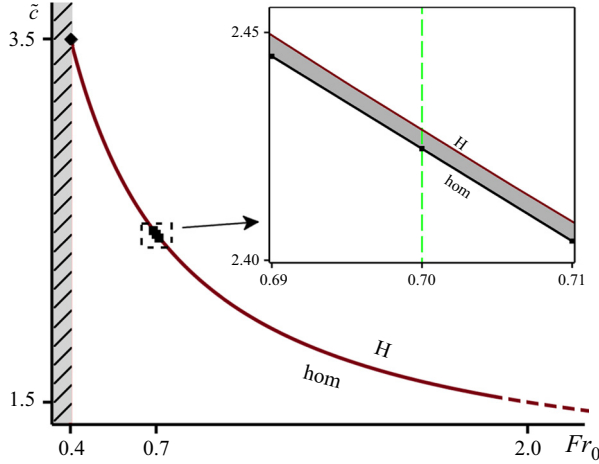
Figure 4. The (Fr_0, \tilde{c}) parameter plane, with the region in which roll waves occur shaded in grey. The upper bound of this region (denoted by ‘H’) is given by (3.2) where the Hopf bifurcation takes place, cf. figure 3, and the lower bound corresponds to the homoclinic event (‘hom’). For Froude numbers below Fr_{cr} = (2/3)(1 - \Gamma) = 0.4 (hatched region) no roll waves exist; the corresponding critical value of \tilde{c} follows from (3.1) and equals 3.5, so the curves ‘H’ and ‘hom’ both emanate from the critical point (Fr_0, \tilde{c}) = (Fr_{cr}, 5/2 + \Gamma/Fr_{cr}) = (0.4, 3.5) . On the scale of the main figure the two curves ‘H’ and ‘hom’ seemingly coincide, therefore we also show an inset in which we magnify the section around Fr_0 = 0.7 (which is one of the typical values used in the text). The system parameters are as in table 1 and the inclination angle of the chute is \zeta = 36^\circ .
