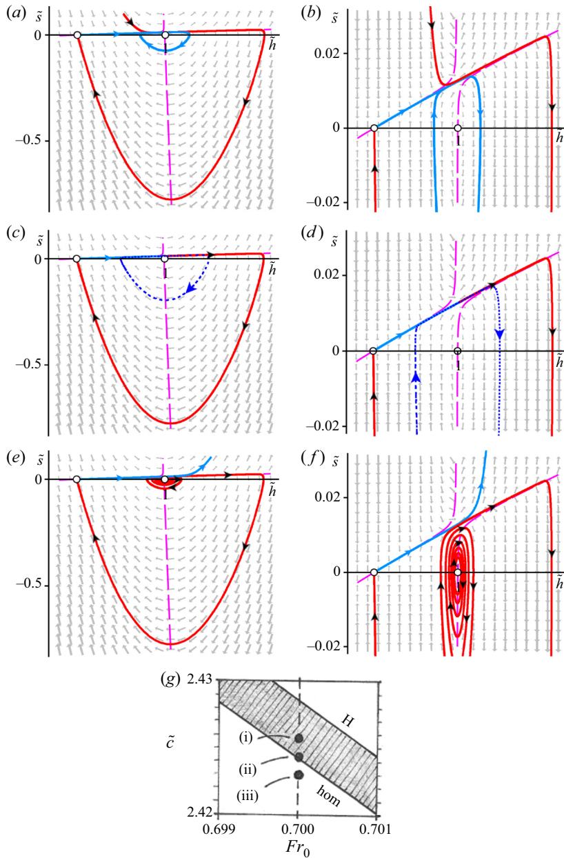
Figure 8. The changing interplay between the stable (red) and unstable (blue) manifolds of the saddle point (\tilde{h}_+, 0) for Fr_0 = 0.7 , at three values of \tilde{c} as shown in the depicted section of the (Fr_0, \tilde{c}) parameter plane. In (b, d, f) , a close-up of the area of interest is given, showing how the interplay determines the fate of the limit cycle. (a, b, g(i)) For \tilde{c}_{hom}(0.7) < \tilde{c} < \tilde{c}_H(0.7) , the unstable manifold (blue curve) is seen to dive below the stable manifold (red curve) and ends on the stable limit cycle surrounding (1, 0) . (c, d, g(ii)) For \tilde{c} = \tilde{c}_{hom}(0.7) , the manifolds join precisely together and form a homoclinic orbit. The maximal size limit cycle has been indicated as a dotted curve. (e, f, g(iii)) For \tilde{c} < \tilde{c}_{hom}(0.7) , the unstable manifold sweeps over the stable one and flies off, whereas the stable manifold now forms a heteroclinic connection between (1, 0) and the saddle (\tilde{h}_+, 0) . The background grey arrows denote the direction field in phase space; the system parameters are as in table 1 and the inclination angle of the chute is \zeta = 36^\circ .
