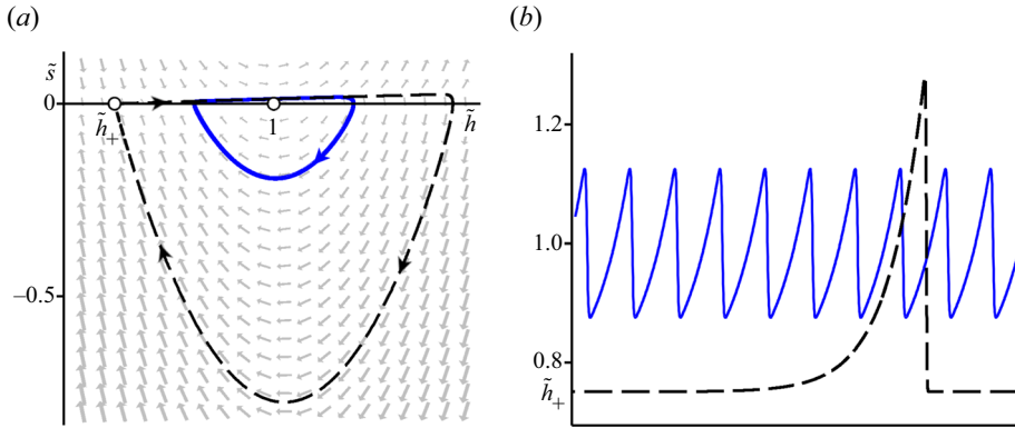
Figure 9. (a) The maximal size limit cycle (solid blue line) and the unstable homoclinic loop (black dashed line) in phase space, cf. figure 8(c,d). (b) The corresponding roll wave train of maximal amplitude (solid blue curve) and the unstable solitary waveform (black dashed curve). The rising flanks of the roll wave train have precisely the same shape as the associated part of the solitary wave. Both these waveforms travel at dimensionless wave speed \tilde{c}_{hom} . The solitary waveform only exists at this very specific value of \tilde{c}_{hom} . For the roll wave train, this same value of \tilde{c}_{hom} is associated with the maximum amplitude the roll waves can attain for the given Froude number Fr_0 . The system parameters are as in table 1 and the inclination angle of the chute is \zeta = 36^\circ ; in view of the extreme fine tuning of \tilde{c} needed to create the homoclinic loop, and since the associated wave profiles are very unstable, the waves presented here have been generated using a value of \tilde{c} marginally larger than \tilde{c}_{hom}(Fr_0) .
