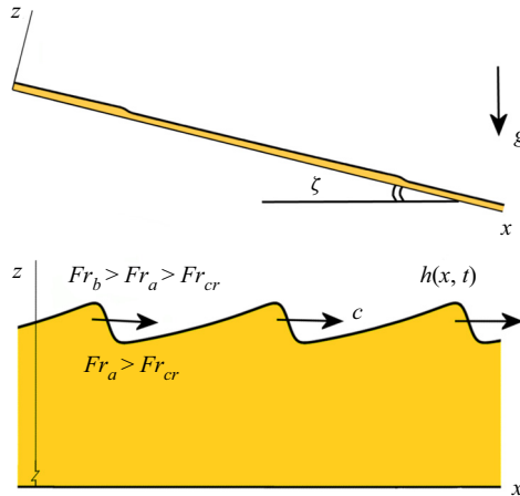
Figure 1. A periodic train of granular roll waves, travelling with wave speed c on a chute with inclination angle \zeta . This is the principal travelling waveform for Froude numbers exceeding the critical value Fr_{cr} given by (1.2). With Fr_b we denote the local Froude number at the crest of the waves, just before the shock front, whereas Fr_a is the Froude number in the trough immediately after the shock front ( Fr_b > Fr_a > Fr_{cr} ). The upper plot depicts the wave profile using identical scaling for the x and z axes, as it will appear in experiment, while the lower plot has been rescaled to demonstrate the features of the wave profile more clearly.
