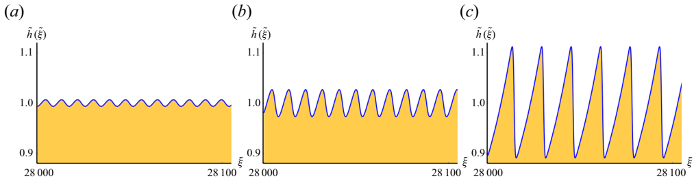
Figure 11. Roll wave profiles for the experimental set-up employed by Rocha et al. (2019), concerning the flow of sand on a chute. The system parameters of this set-up are given in table 2. The inclination angle of the chute is \zeta = 34^\circ and the Froude number of the incoming flow is Fr_0 = 0.7 , well above the critical value Fr_{cr} = 0.107 for this set-up. The depicted wave profiles correspond to three successive values of the wave speed: (a) \tilde{c} = \tilde{c}_H - 0.5 \times 10^{-4} , (b) \tilde{c} = \tilde{c}_H - 7.0 \times 10^{-4} and (c) \tilde{c} = \tilde{c}_H - 24.28 \times 10^{-4} , where \tilde{c}_H = 2.42857 marks the birth of the roll waves.
