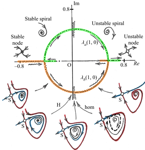
Figure 3. The trajectories in the complex plane, for decreasing \tilde{c} and at a fixed Froude number Fr_0 = 0.7 , of the two eigenvalues \lambda_{a,b}(1, 0) of the fixed point (\tilde{h}, \tilde{s}) = (1, 0) . In the insets above the main plot we sketch how the local stability characteristics of the fixed point (1, 0) change as the eigenvalues vary. The five schematic pictures below the main plot depict how, simultaneously, the orbits surrounding the fixed point (1, 0) interact with those around the neighbouring saddle point (\tilde{h}_+, 0) denoted by ‘S’. The stable and unstable manifolds of the latter are indicated in red and blue, respectively. The letter ‘H’ stands for Hopf bifurcation (where (1, 0) is momentarily a centre point and gives birth to a limit cycle) and ‘hom’ denotes the critical event where the stable and unstable manifolds of the saddle connect to form a closed homoclinic loop. In the region between ‘H’ and ‘hom’ (dashed) the fixed point (1, 0) is surrounded by a stable limit cycle, see the middle picture below the main plot; this limit cycle corresponds to a periodic train of roll waves.
