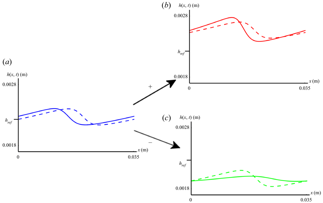
Figure 12. Evolution of the roll wave profiles for different values of the influx, i.e. different values of the Froude number Fr_0 . Depicted are the profiles after 10 s (solid lines) together with the initial profiles (dashed lines) for: the reference Froude number Fr_0 = 0.70 (a), increased Froude number Fr_0 = 0.77 (b) and reduced Froude number Fr_0 = 0.59 (c). We have imposed periodic boundary conditions, with domain length equal to the wavelength of the reference wave. The system parameters are as in table 1 and the inclination angle of the chute is \zeta = 36^\circ .
