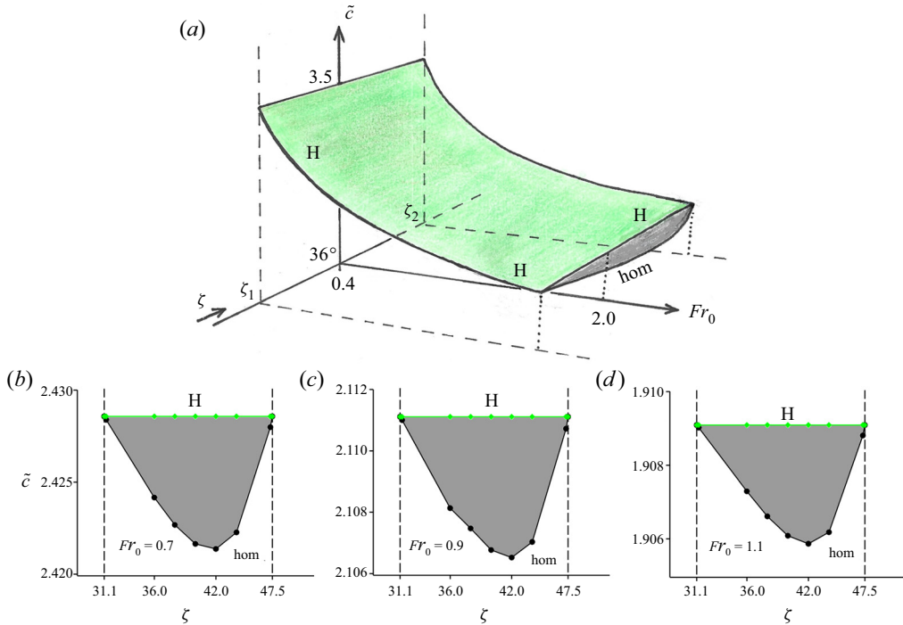
Figure 10. The three-dimensional (Fr_0, \tilde{c}, \zeta) parameter space, being an extension of the (Fr_0, \tilde{c}) plane shown in figure 4, with the region in which roll waves occur shaded in grey. The upper bound of this region (the green surface denoted by ‘H’, where the roll waves are born via a Hopf bifurcation) is given by (3.2); the lower bound ‘hom’ is where the roll waves attain their maximal size, which is determined by the homoclinic event as shown in figure 7. The three plots in the lower row depict the region in question – with the numerically calculated values of ‘hom’ – for three cuts through the three-dimensional plot at Fr_0 = 0.7, 0.9 , and 1.1 ; note the different scaling along the \tilde{c} -axis in these plots. The system parameters are as in table 1.
