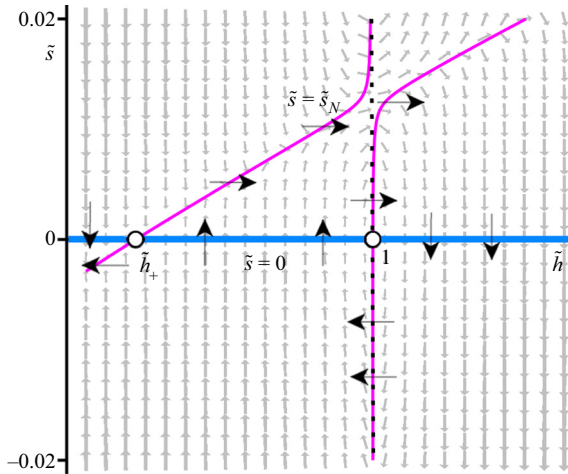
Figure 2. The fixed points (\tilde{h}_+, 0) and (1, 0) (indicated by open dots) in the (\tilde{h}, \tilde{s}) phase plane for Fr_0 = 0.7 and \tilde{c} = 2.42457 (= \tilde{c}_H - 0.004) , together with the vertical-motion nullcline \tilde{s} = 0 (blue) and the horizontal-motion nullcline \tilde{s} = \tilde{s}_N (magenta, given by (2.26)). The black dotted line depicts the almost vertical contour of zero divergence of the vector field, which is discussed in § 3.3. The grey background arrows denote the direction field of the dynamical system and the large black arrows signify this field evaluated on the nullclines. The system parameters are as in table 1 and the inclination angle is chosen to be \zeta = 36^\circ .
