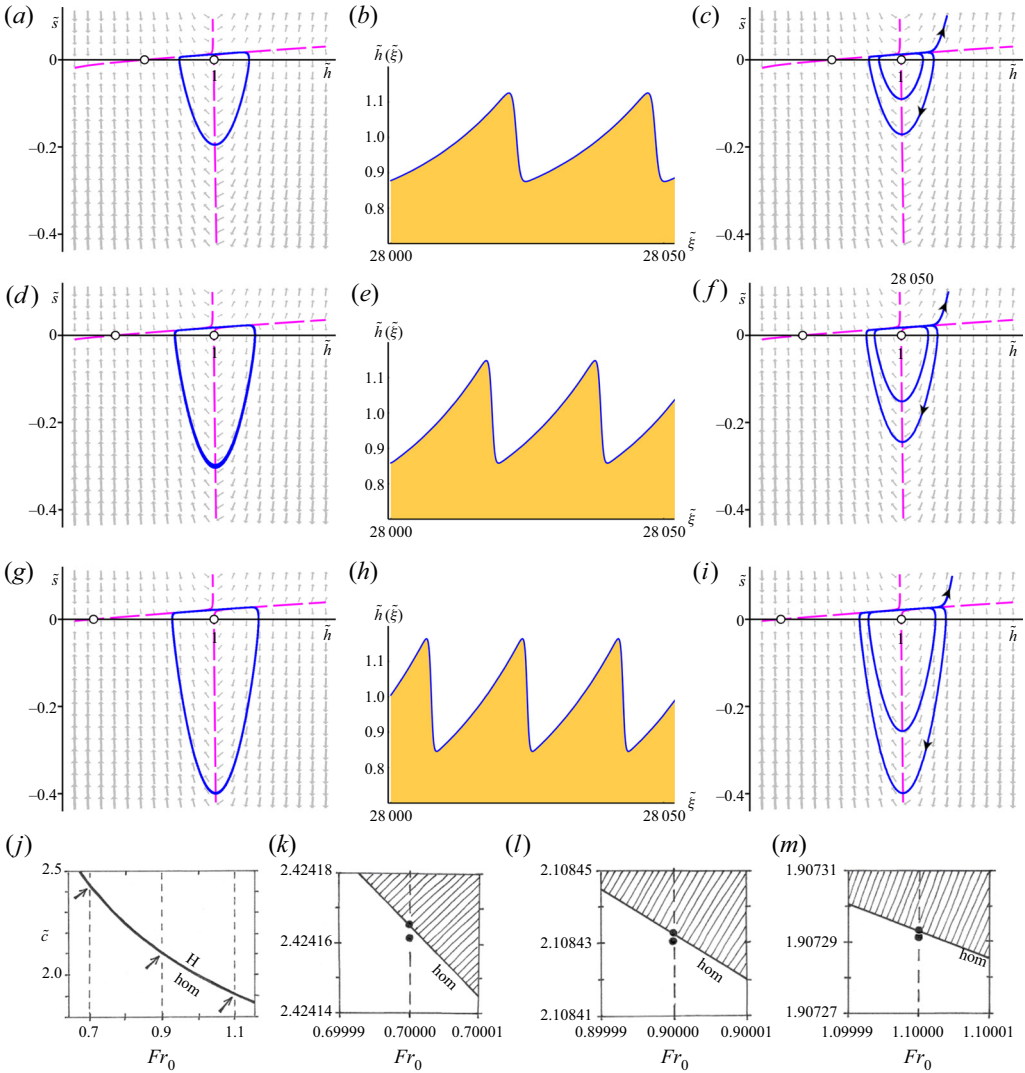
Figure 7. (a,d,g) The maximal size limit cycles in phase space (blue solid curves) along with the two branches of the horizontal-motion nullcline \tilde{s} = \tilde{s}_N (magenta curves) for Froude numbers Fr_0 = 0.7 , Fr_0 = 0.9 and Fr_0 = 1.1 , respectively. The corresponding wave speeds are \tilde{c}_{hom}(0.7) = \tilde{c}_H(0.7) - 0.004406 \simeq 2.424165 , \tilde{c}_{hom}(0.9) = \tilde{c}_H(0.9) - 0.002679 \simeq 2.108432 and \tilde{c}_{hom}(1.1) = \tilde{c}_H(1.1) - 0.00179804 \simeq 1.907293 . (b,e,h) The associated fully ripened wave profiles. (c,f,i) ‘Escape’ of the limit cycles (through the gap between the two branches of the horizontal-motion nullcline) for \tilde{c} -values that are just below the aforementioned critical ones, namely: \tilde{c} = 2.424161 for Fr_0 = 0.7 , \tilde{c} = 2.108431 for Fr_0 = 0.9 and \tilde{c} = 1.907292 for Fr_0 = 1.1 . The above choices of Fr_0 and \tilde{c} are indicated in the (Fr_0, \tilde{c}) diagram in (j–m), the regions marked by the arrows in the first plot are given in more detail in the three magnifications to the right. The other parameters are invariably taken as in table 1 and the inclination angle is \zeta = 36^\circ .
