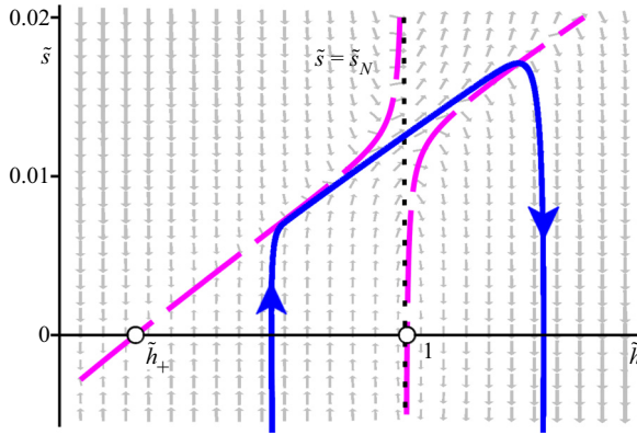
Figure 6. The path traced out by the limit cycle (solid blue curve) in the upper half-plane is seen to closely follow a path in the immediate vicinity of the two branches of the horizontal-motion nullcline \tilde{s} = \tilde{s}_N (magenta dashed curves, given by (2.26)). In fact, the vector field forces all trajectories in this region through a narrow channel around the left branch until they cross the contour of zero divergence (dotted), after which they start to drift apart. Subsequently, the limit cycle crosses the right branch of the horizontal-motion nullcline and curves downwards. The background grey arrows denote the direction field of the dynamical system; the parameters are as in table 1 and the inclination angle is \zeta = 36^\circ .
