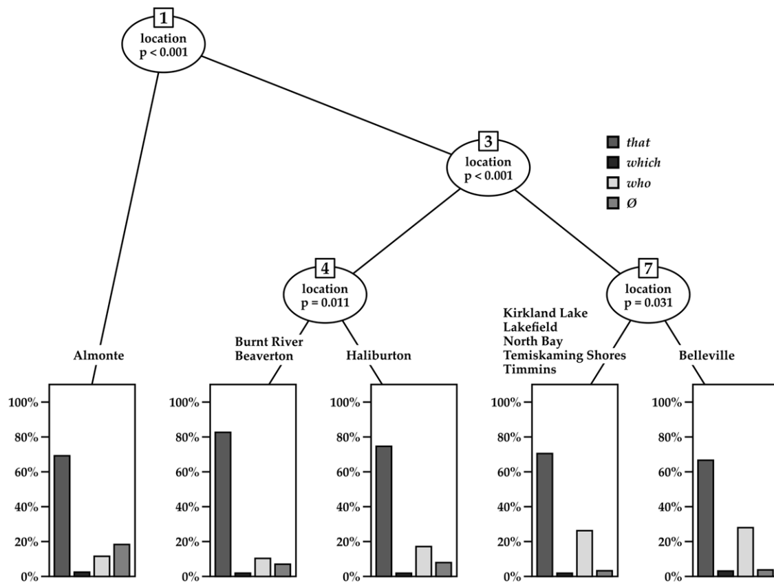
Figure 2. Conditional inference tree (Hothorn et al., 2006) conducted in R 3.6.3 (R Core Team, 2020).
