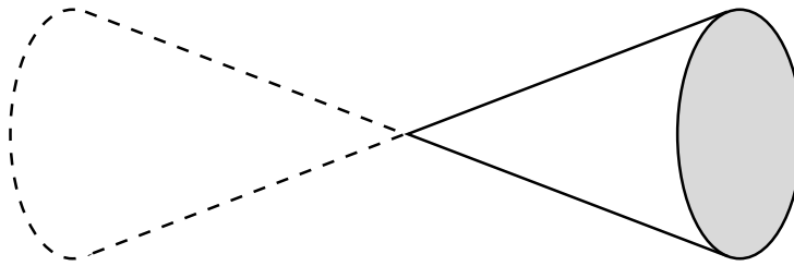
Figure 1. In solid lines: the quotient of the real analytic manifold \mathbb{R}^2 by the linear group action of \{\pm 1\} , embedded in \mathbb{R}^3 as the semicone w^2 = uv, u \geq 0, v \geq 0 . The embedding is given by (u, v, w) = (x^2, y^2, xy) .
