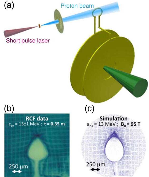
Figure 6. Example of a proton deflectometry measurement: (a) schematic of the setup; (b) image obtained on RCF with 13 MeV protons; (c) simulation of proton deflection in a B -field [35] .
