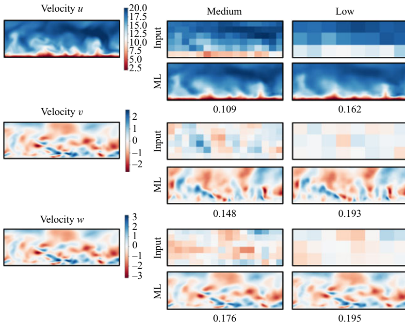
FIGURE 13. Velocity contours at a y - z section ( x^+ = 1127 ) of the reference DNS data, coarse input data and the recovered flow field through spatial SR analysis with machine learning (ML). The values listed below the contours are the L_2 error norm \epsilon .
