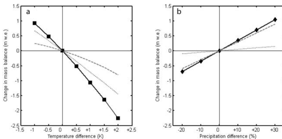
Fig. 7. Sensitivity of the mass balance of Engabreen to changes in (a) temperature and (b) precipitation. Filled symbols connected by black lines are associated net mass balance; effects on winter (dashed line) and summer (dotted line) mass balances are shown in grey.
