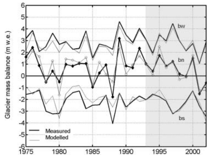
Fig. 5. The temporal evolution of mass balance of Engabreen. Values of winter ( b_w ), summer ( b_s ) and net ( b_n ) mass balances are shown separately. The shaded area indicates the calibration period.
