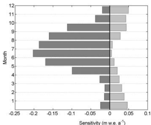
Fig. 6. Seasonal sensitivity characteristic of Engabreen. Values represent the sensitivity of the annual mass balance to monthly perturbations in temperature (dark grey) and precipitation (light grey).
