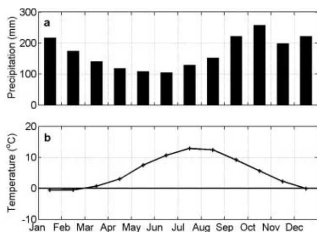
Fig. 2. Mean values of monthly precipitation sums (a) and average air temperature (b) as recorded at the meteorological station Glomfjord, 1974–2002.
