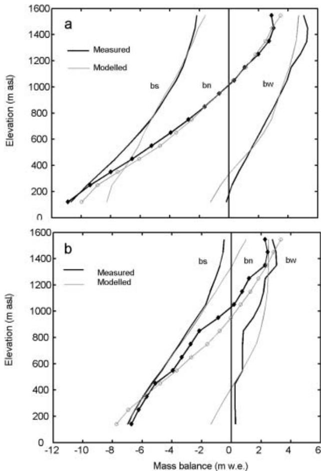
Fig. 4. Examples of mass-balance profiles (a) for a good (1997) and (b) for a less satisfying (1982) agreement between simulations (grey lines) and measurements (black lines). Profiles are shown of winter mass balance ( b_w ), summer balance ( b_s ) and net mass balance ( b_n ).
