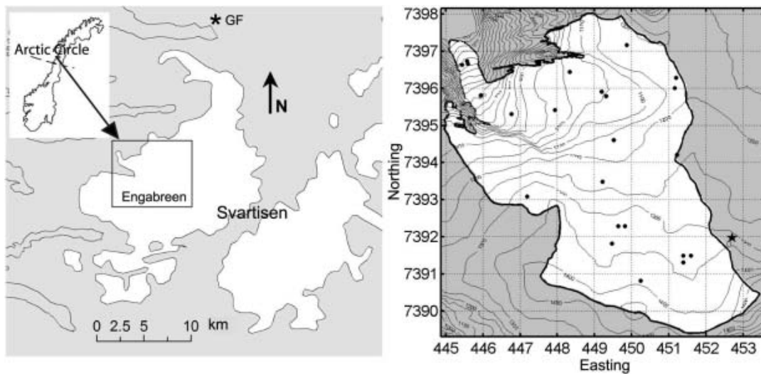
Fig. 1. Location maps of Engabreen and Svartisen ice cap in northern Norway (left). The star indicates the location of the meteorological station Glomfjord (GF). Dots in the map on the right mark the approximate position of mass-balance stakes, and the star denotes the location of the automatic weather station Skjæret. Grid zone is UTM 33 and units are kilometres.
