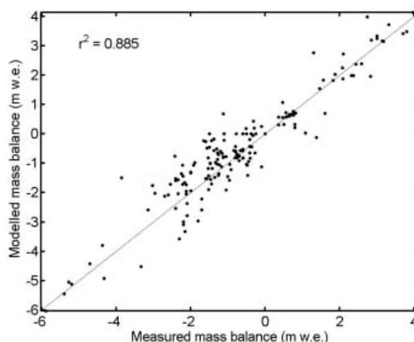
Fig. 3. Scatter plot of measured vs calculated mass balance at individual stakes. The number of samples is 174.
