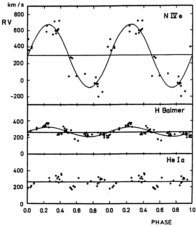
Fig. 2. Observed radial velocities of Sk-67°18 for the N IV 4058Å emission and the H Balmer and He I \alpha absorption.
