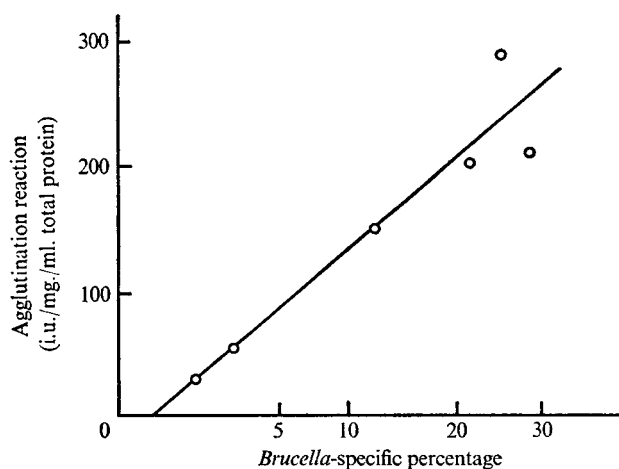
Fig. 2. Dependence of serum agglutination test activity of IgG 1 preparations on the Brucella -specific percentage. The regression line is described by the equation Y = 8.50x - 19.1 , where Y is the international units per mg. per ml. of total protein and x is the Brucella -specific percentage after angular transformation.
