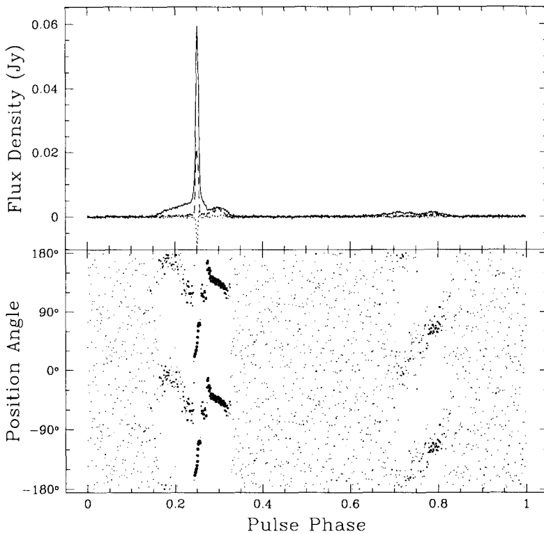
Figure 2. The 1400 MHz pulse profile of PSR B1534+12. The solid, dashed and dotted lines indicate total, linear and circular power, respectively. The polarization position angle is shown in the lower panel.
