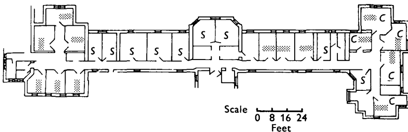
Fig. 1. Plan of the isolation ward. Bedrooms marked C have a ducted cool air supply as well as the individual room ventilator. S = service rooms, including offices and kitchen.
