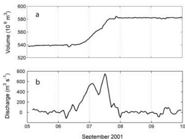
Fig. 3. (a) Inflow to the reservoir Sisovatr prior to and during the jökulhlaup; and (b) the reconstructed hydrograph.
