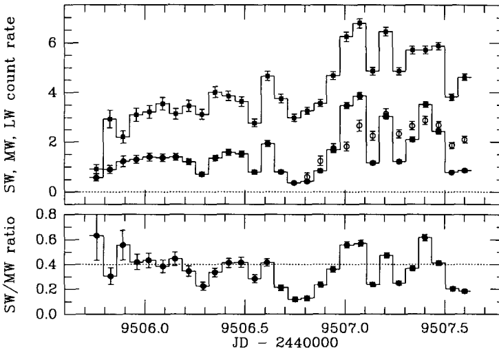
Figure 1. Upper panel: SW (100...170 Å: filled circles), MW (170...300 Å: filled squares), and LW (300...400 Å: open circles) count rate light curves of VW Hyi. Lower panel: SW over MW (hard over soft) count rate ratio.
