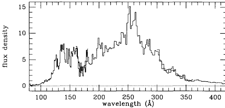
Figure 2. Net SW (80...180 Å), MW (160...360 Å) and LW (300...420 Å) spectra of VW Hyi. Units of flux density are 10^{-12} erg \text{cm}^{-2} \text{s}^{-1} Å ^{-1} .
