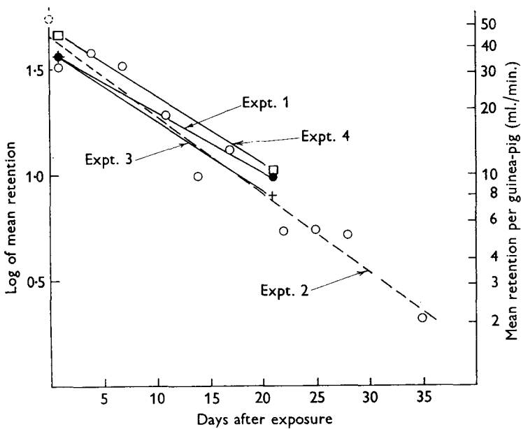
Fig. 1. Retention of airborne radioactive bacterial spores in lower respiratory tract of guinea-pig, measured at various times after inhalation. ○ is zero time, Expt. 2, (not used in calculations).
