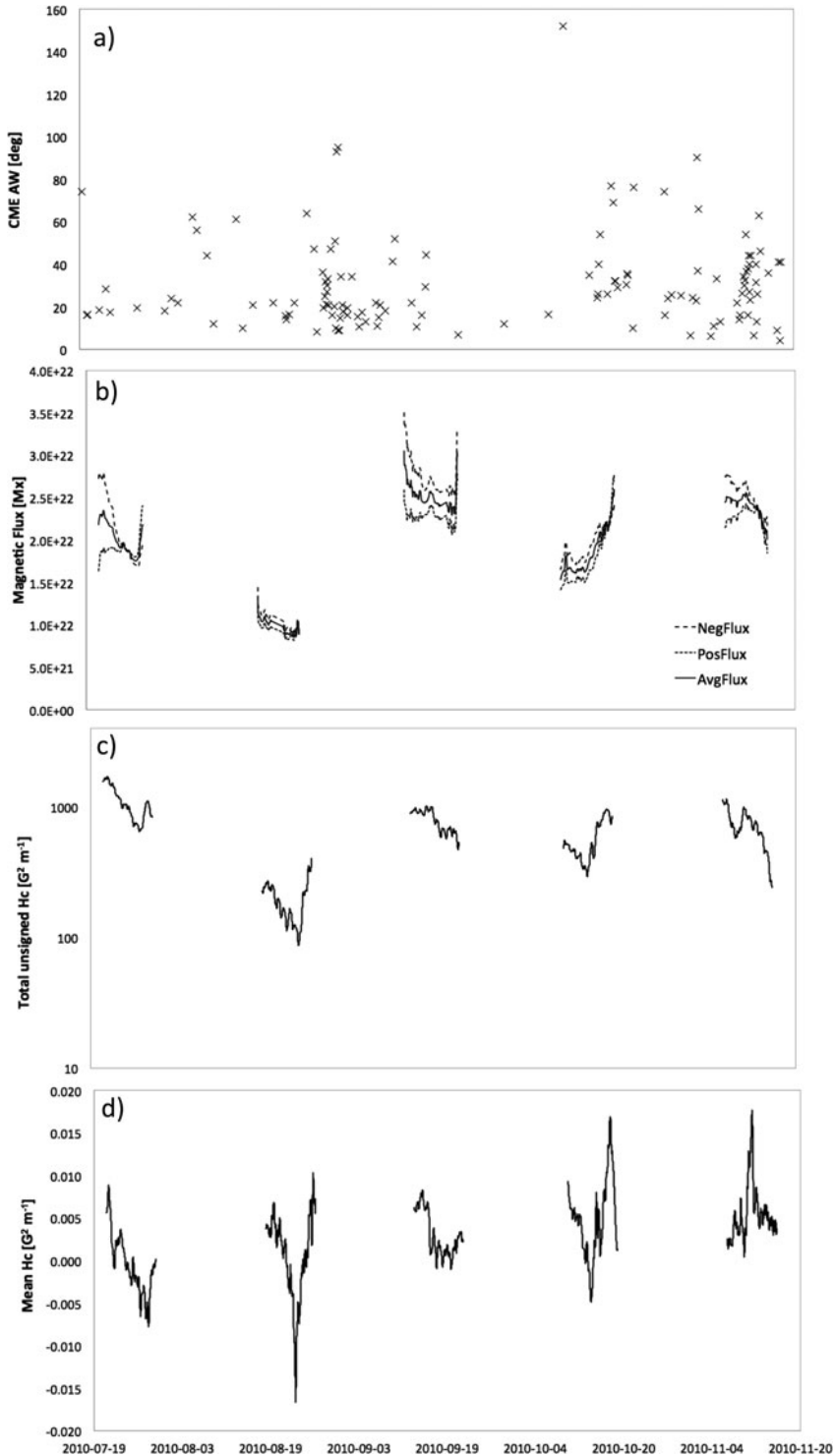
Figure 1. Temporal behavior of the eruptive activity and magnetic parameters associated with the active region during the investigated time interval. a) CME AW. b) Average magnetic flux (solid line), positive magnetic flux (dotted line), and negative magnetic flux (dashed line). c) Total unsigned current helicity H_c , in a logarithmic scale. d) Mean current helicity.
