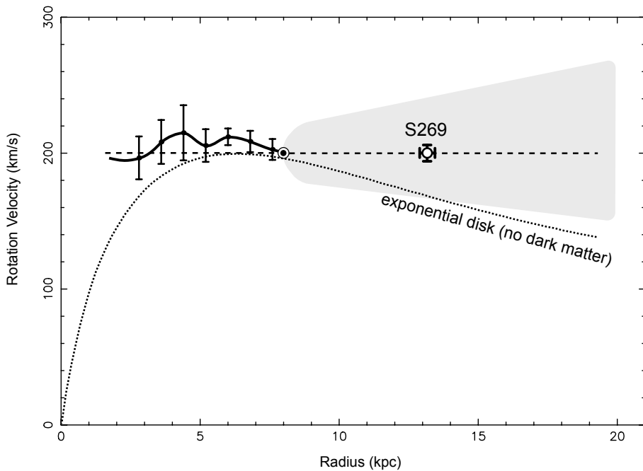
Figure 2. Rotation curve of the Galaxy obtained in the previous studies as well as the result from S269 using Galactic constants of R_0=8 kpc and \Theta_0=200 km ^{-1} . The dashed line is the flat rotation curve with \Theta=200 km ^{-1} , and the shadowed area shows the possible range of outer rotation curves in previous studies (Honma & Sofue 1997). Points at R \leq 8 kpc are inner rotation curves determined from the tangential velocities of Galactic HI gases (Honma & Sofue 1997), with a smoothed fit (thick curve). The dotted curve is the rotation curve for an exponential disk, corresponding to a constant mass-to-light ratio disk without dark matter. The discrepancy between the observed point for S269 and the exponential disk is evident, demonstrating the existence of large amount of dark matter in the outer region of the Galaxy.
