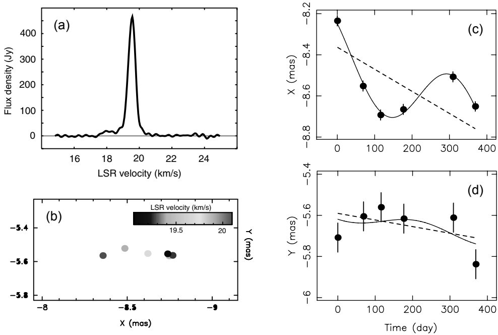
Figure 1. (a, top left) Auto-correlation spectrum of S 269 H 2 O maser emissions taken on DOY 073 in 2005. (b, bottom left) maser spot distribution obtained with VERA on DOY 073 in 2005. The coordinates are with respect to the tracking center position, which is (06h14m37.08s, +13d49'36.7") in J2000. (c, top right) Positional variations of the brightest maser spot at V_{\text{LSR}}=19.6 \text{ km s}^{-1} for X (east-west) direction. (d, bottom right) the same plot for Y (north-south) direction. The time origin is the first epoch of our observations, which is DOY 323 in 2004. Solid curves are best-fit results with parallax and proper motions, and dashed lines show the best-fit proper motions.
