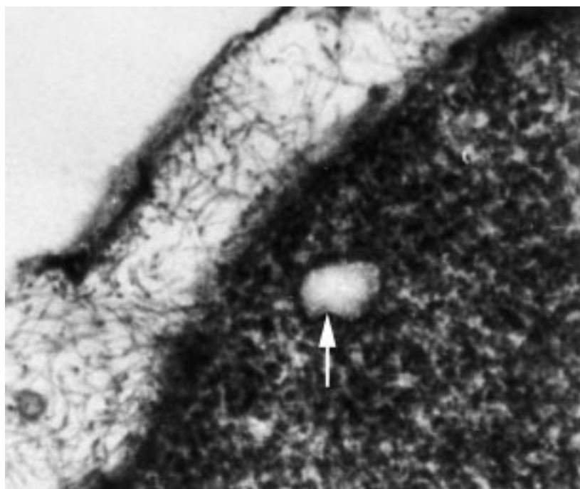
Fig. 4. Transmission electron micrograph of human lens epithelium cells incubated for 72 h in growth medium supplemented with 30 mM-galactose and 10\ \mu\text{M} -lycopene (magnification \times 15\,000 ). \uparrow , Vacuoles decrease in number and size; |-| , 0.4\ \mu\text{m} . For details of procedures, see p. 348.
