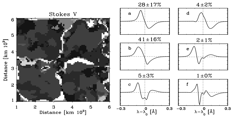
Figure 1. Left panel: map of the classes of the FeI 6302 Å Stokes V profiles. The grey scaling from black to white corresponds to the change of the zero-crossing shift of the class profiles from red to blue accompanied by the change of the area asymmetry from negative to positive. The locations of the irregular profiles are marked by the lightest colors. Right panel: examples of class profiles. The fraction of line profiles belonging to each class is given in percent at the top of each panel.
