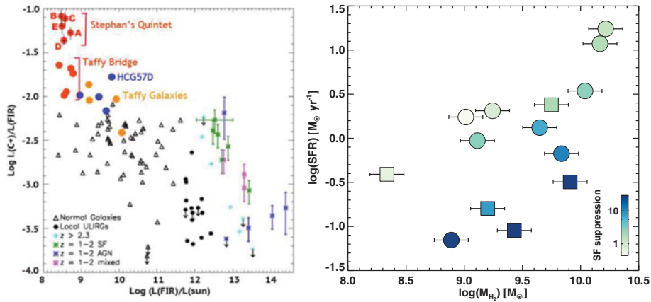
Figure 3. (Left): The L([C II])/L_{FIR} vs L_{FIR} of starforming galaxies and ULIRGs (Malhotra et al. 2001) and high- z sources (Stacey et al. 2010). There is an approximate L([C II])/L_{FIR} upper limit of 1%, until we include sources known to have shocks, including the Taffy Galaxies (Peterson et al. 2012), Stephan’s Quintet (Appleton et al. 2013) and HCG 57 (Alatalo et al. 2014b). (Right): The total star formation rate calculated from Bitsakis et al. (2014), normalized to a Salpeter initial mass function (Salpeter 1955) compared to the molecular gas mass derived from the CO(1–0) data from CARMA (using the L_{CO} –to– M_{H_2} conversion of 2. \times 10^{20} \text{ cm}^{-2} (\text{K km s}^{-1})^{-1} ; Bolatto et al. 2013). The colorization is based on the distance off of the relation derived in Kennicutt (1998).
