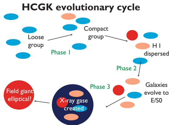
Figure 1. A schematic of the proposed HCG evolutionary picture. The H I observations taken by Verdes-Montenegro et al. (2001) and Borthakur, Yun & Verdes-Montenegro (2010) support the Hickson (1997) picture in which galaxies start in a loose group, move into the compact group phase (during which the H I in the individual galaxies are dispersed) until the gas is located within a common envelope. During the evolution of the ISM, the galaxies within the group are also transitioning (Johnson et al. 2007; Walker et al. 2010, 2013; Cluver et al. 2013).
