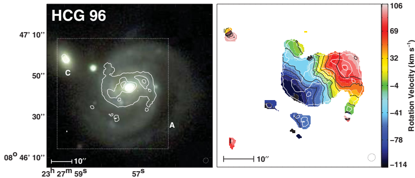
Figure 2. An example of the CO data from CARMA. (Left): The Sloan Digital Sky Survey g, r, i image underlies the moment0 map of HCG 96a and 96c (labeled on the diagram), which were both detected in the CARMA pointing. (Right): The mean velocity map of HCG 96a and 96c. In HCG 96a, the velocity structure traces the spirals, and in HCG 96c, the molecular gas is centralized, and regularly rotating.
