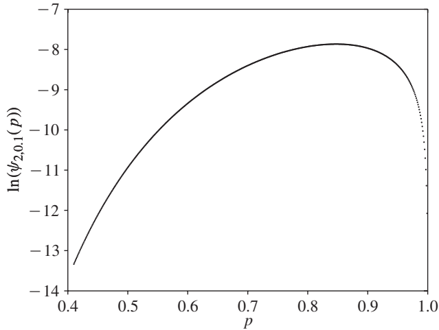
FIGURE 1: Plot of \ln(\psi_{2,0.1}(p)) against p for the 51-out-of-100 system.
