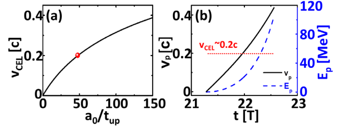
Figure 2. (a) Relation between the velocity of the compressed electron layer v_{\text{CEL}} and the steepness of the laser front a_0/t_{\text{up}} according to Equation (5) for n_0 = 50n_c . (b) Evolutions of the velocity, v_p (black solid line), and energy, E_p , of the proton layer during the HB stage.
