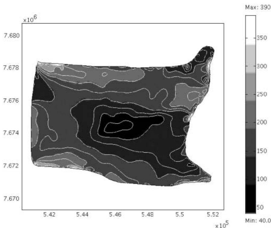
Fig. 12. The effective stress field on the floating portion of Jakobshavn Isbræ computed from results of the uncrevassed ice-shelf experiment. Units are kPa. Contours are spaced at 25 kPa. There are no high-stress regions that propagate transversely across this ice, indicating that continuum mechanics fails to capture all the dynamics of this system.
