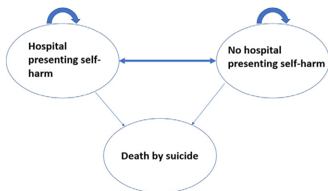
Figure 1. Overview of three-state Markov model.
