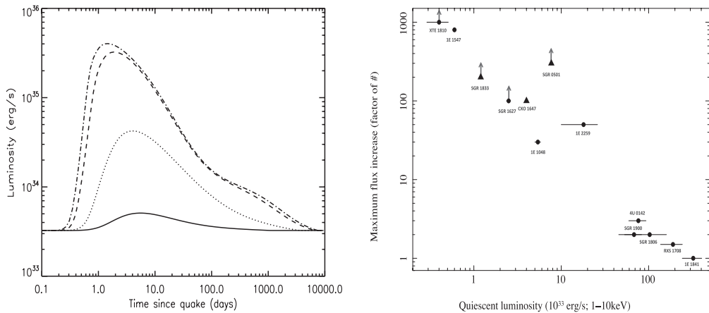
Figure 3. Left: Luminosity vs. time after energy injection. The models correspond to E_{oc} = 1.7 \times 10^{41} erg, (solid line), 1.7 \times 10^{42} erg (dotted line), 1.7 \times 10^{43} erg (dashed line), and 1.7 \times 10^{44} erg (dash-dotted line). Right: quiescent luminosity vs. outburst maximum flux increase (all in the 1-10 keV band), for all magnetars showing bursts, glitches or outbursts. See Pons & Rea 2012 for further details.
