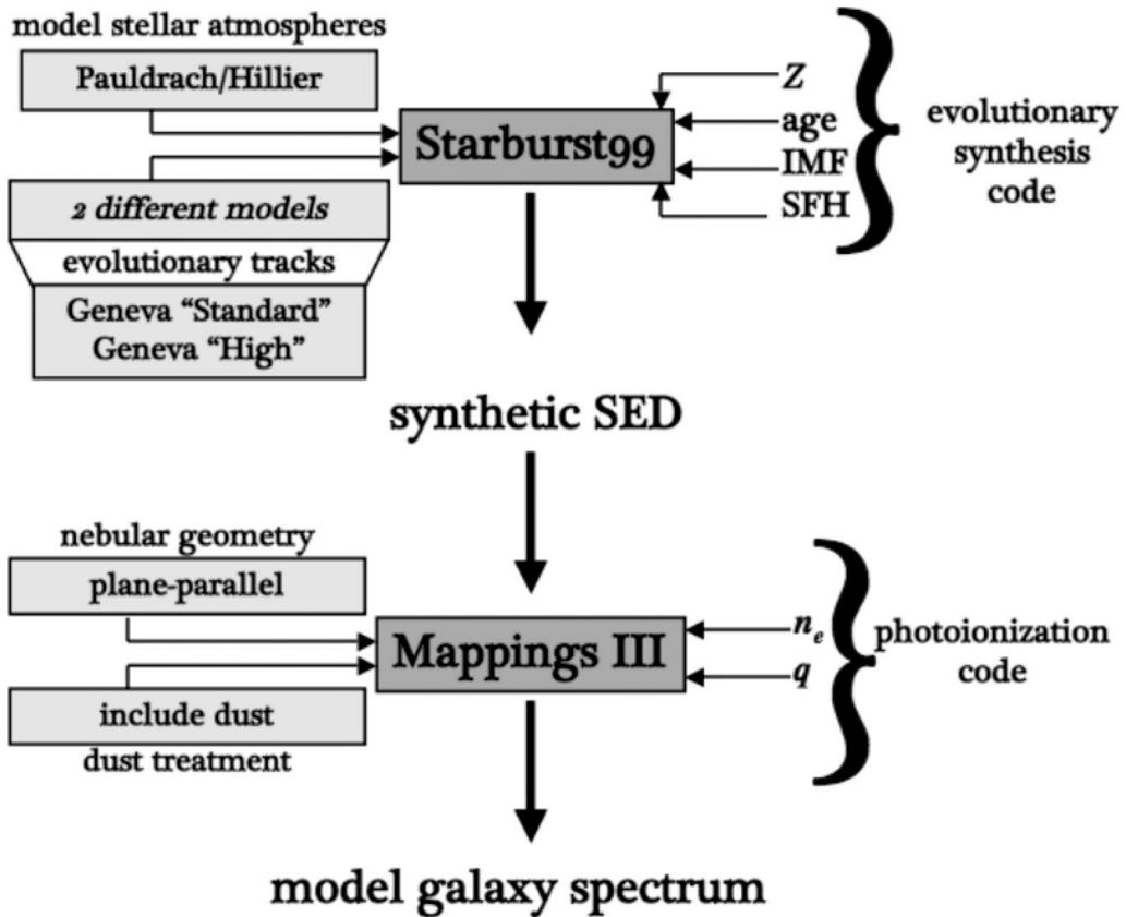
Figure 1. Illustration of the inputs taken by the Starburst99 and Mappings III codes when generating our model grids.
