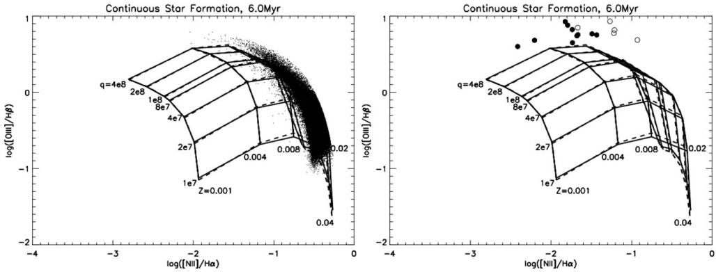
Figure 2. [NII]/H \alpha vs. [OIII]/H \beta emission line diagnostic grids for a 6.0 Myr continuous star formation model grid; an electron density of 100 is assumed. Left: the grid is in excellent agreement with the position of 60,920 SDSS star-forming galaxies (small points). Right: the agreement of the grid with the MPGs (filled circles), and LGRB hosts (open circles). We see that the models are in poor agreement with the MPG and LGRB host samples. In the electronic color version of these figures, lines of constant metallicity are shown in blue/green, while lines of constant ionization parameter are shown in red/yellow.
