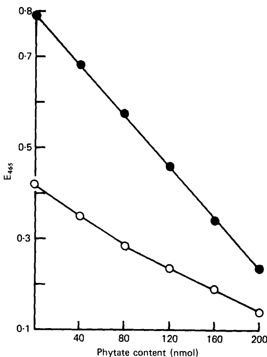
Fig. 1. A comparison of the standard curves relating phytate content (nmol) and extinction at 465 nm ( E_{465} ) using the original aqueous Holt (1955) procedure (○—○) and the modified assay (●—●), as described on p. 580.
